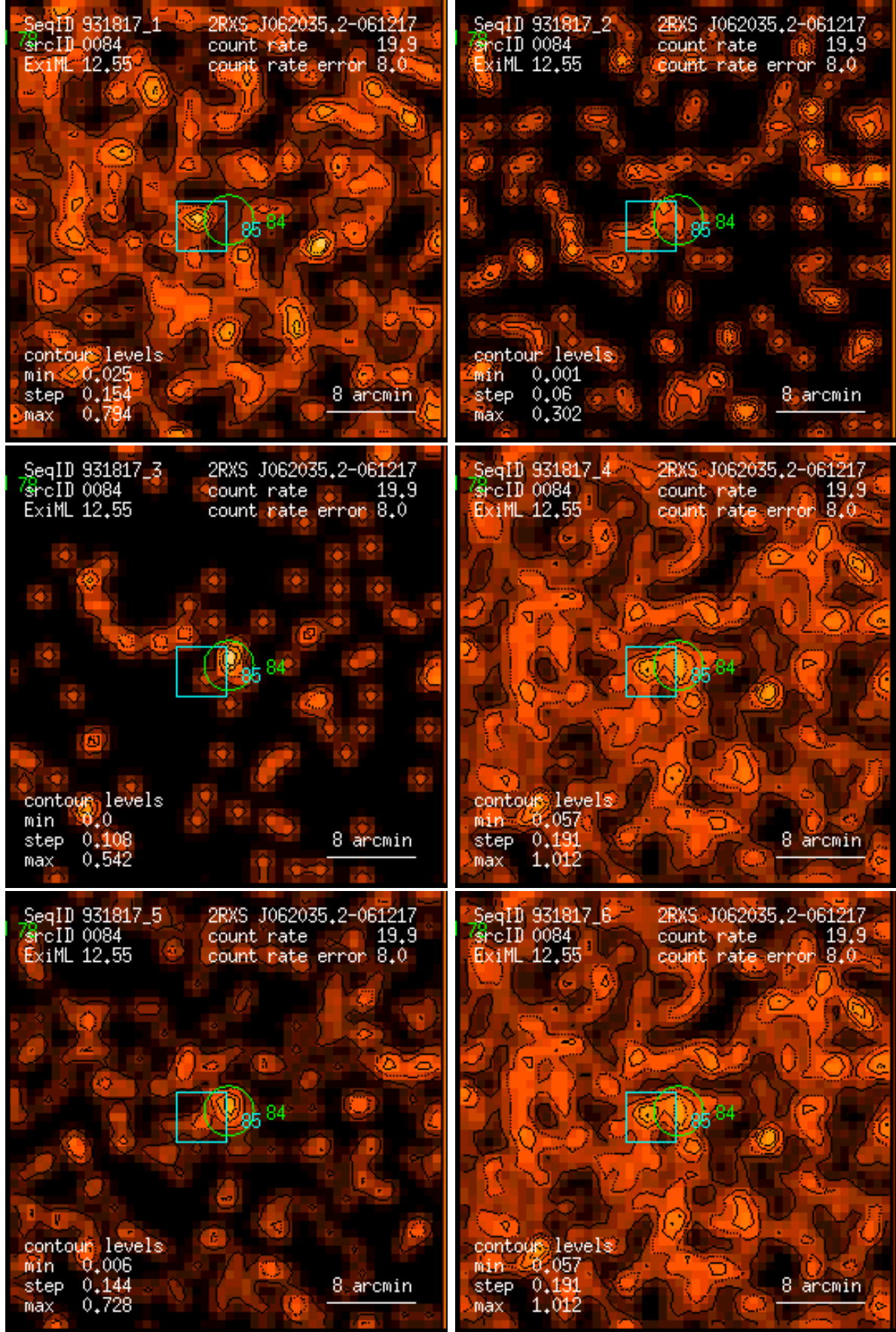
Figure 84: RASS 931817: detection 0084: band rate images, Gaussian filter: (1) PSPC channels 11 – 41, (2) 52 – 90, (3) 91 – 201, (4) 11 – 235, (5) 52 – 201, (6) 11 – 201. Broad band rates in counts/ks. Band rate contour levels in counts/ks/arcmin 2 .
