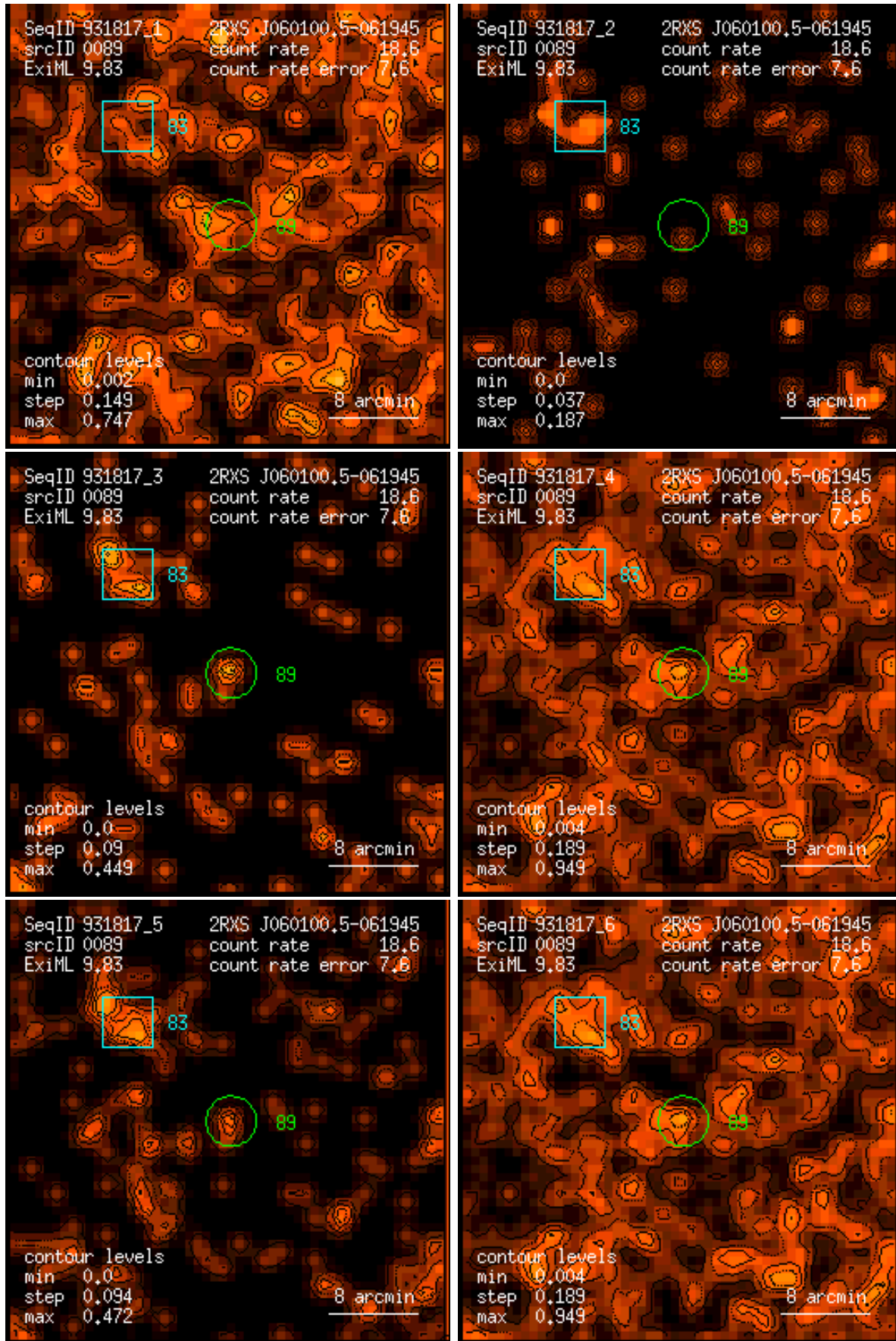
Figure 89: RASS 931817: detection 0089: band rate images, Gaussian filter: (1) PSPC channels 11 – 41, (2) 52 – 90, (3) 91 – 201, (4) 11 – 235, (5) 52 – 201, (6) 11 – 201. Broad band rates in counts/ks. Band rate contour levels in counts/ks/arcmin 2 .
