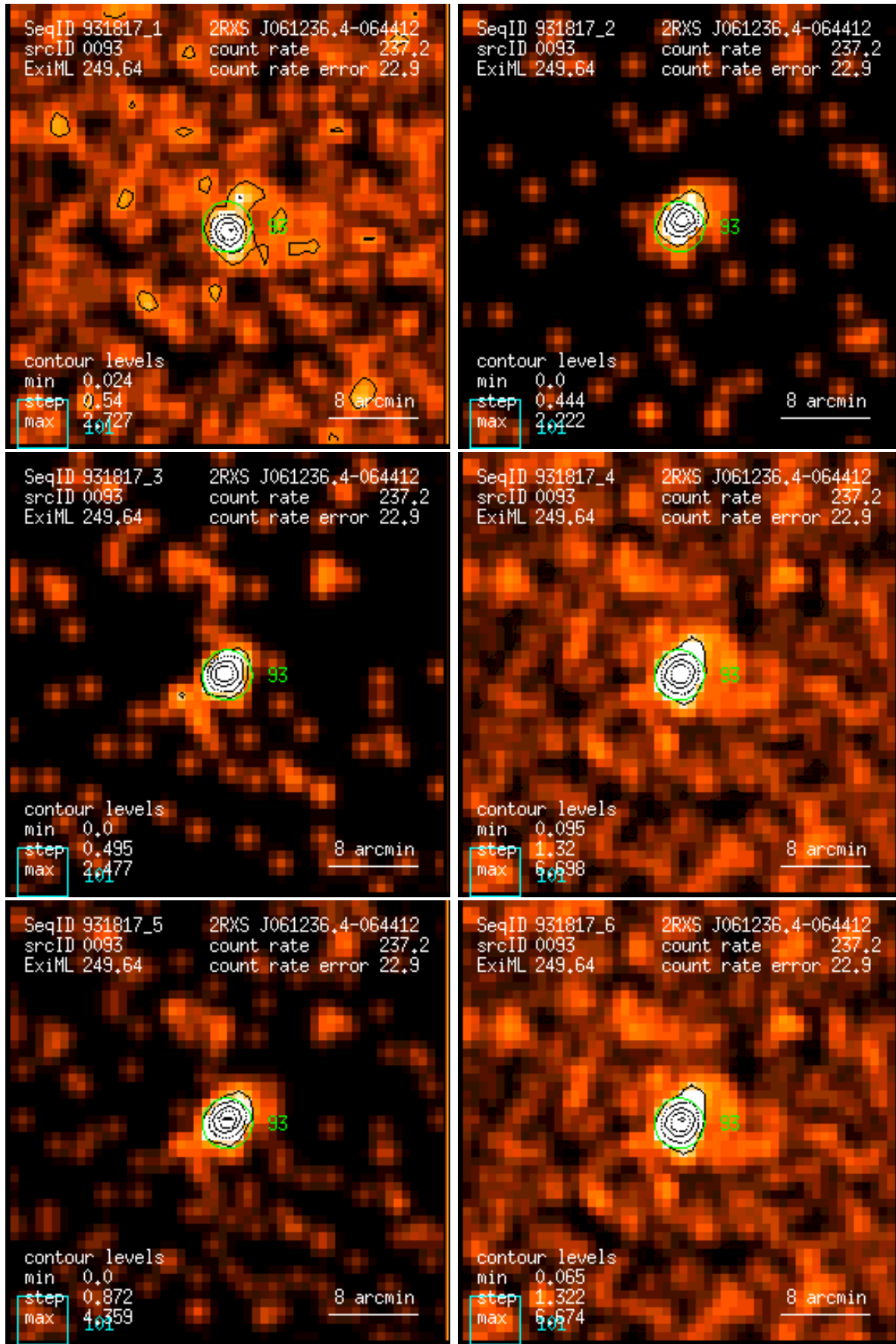
Figure 93: RASS 931817: detection 0093: band rate images, Gaussian filter: (1) PSPC channels 11 – 41, (2) 52 – 90, (3) 91 – 201, (4) 11 – 235, (5) 52 – 201, (6) 11 – 201. Broad band rates in counts/ks. Band rate contour levels in counts/ks/arcmin 2 .
