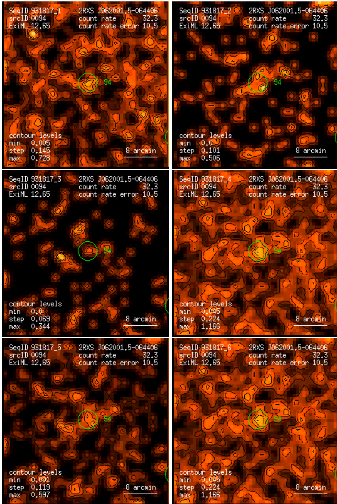
Figure 94: RASS 931817: detection 0094: band rate images, Gaussian filter: (1) PSPC channels 11 – 41, (2) 52 – 90, (3) 91 – 201, (4) 11 – 235, (5) 52 – 201, (6) 11 – 201. Broad band rates in counts/ks. Band rate contour levels in counts/ks/arcmin 2 .
