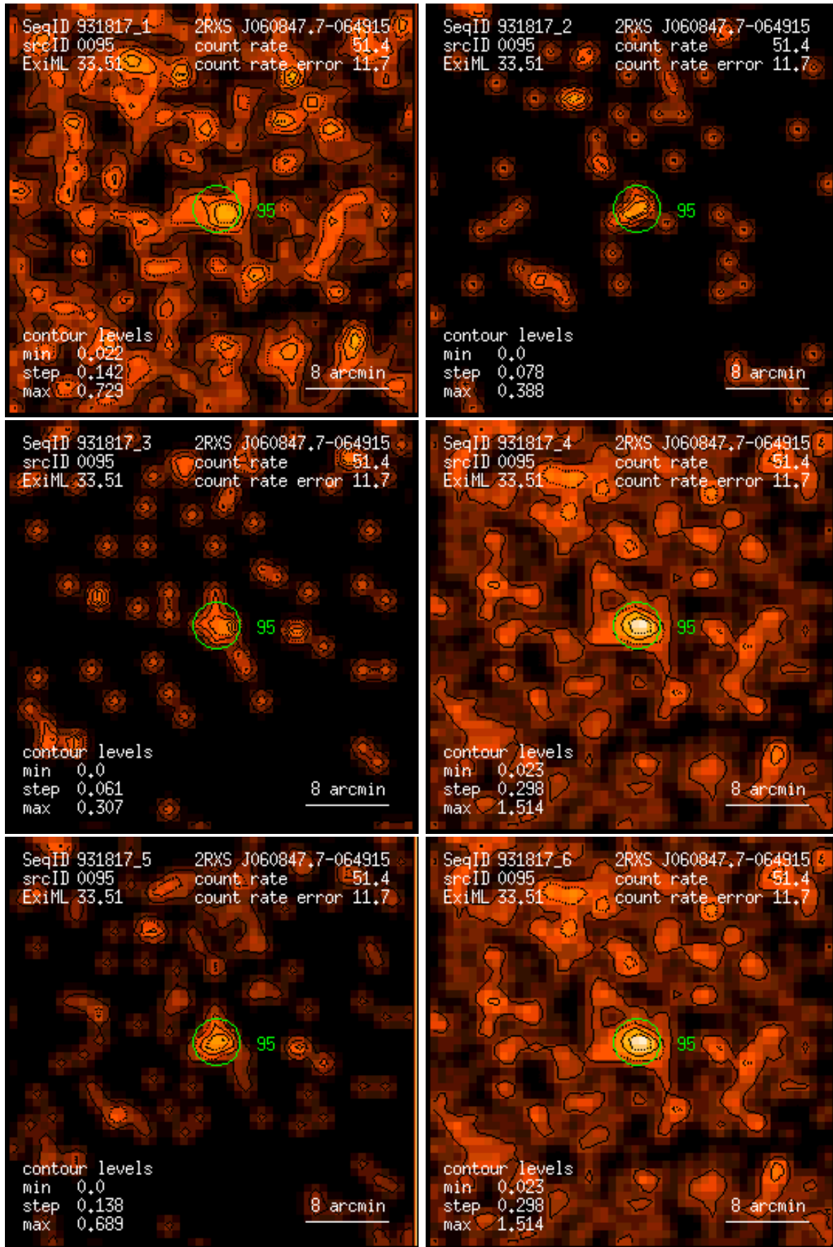
Figure 95: RASS 931817: detection 0095: band rate images, Gaussian filter: (1) PSPC channels 11 – 41, (2) 52 – 90, (3) 91 – 201, (4) 11 – 235, (5) 52 – 201, (6) 11 – 201. Broad band rates in counts/ks. Band rate contour levels in counts/ks/arcmin 2 .
