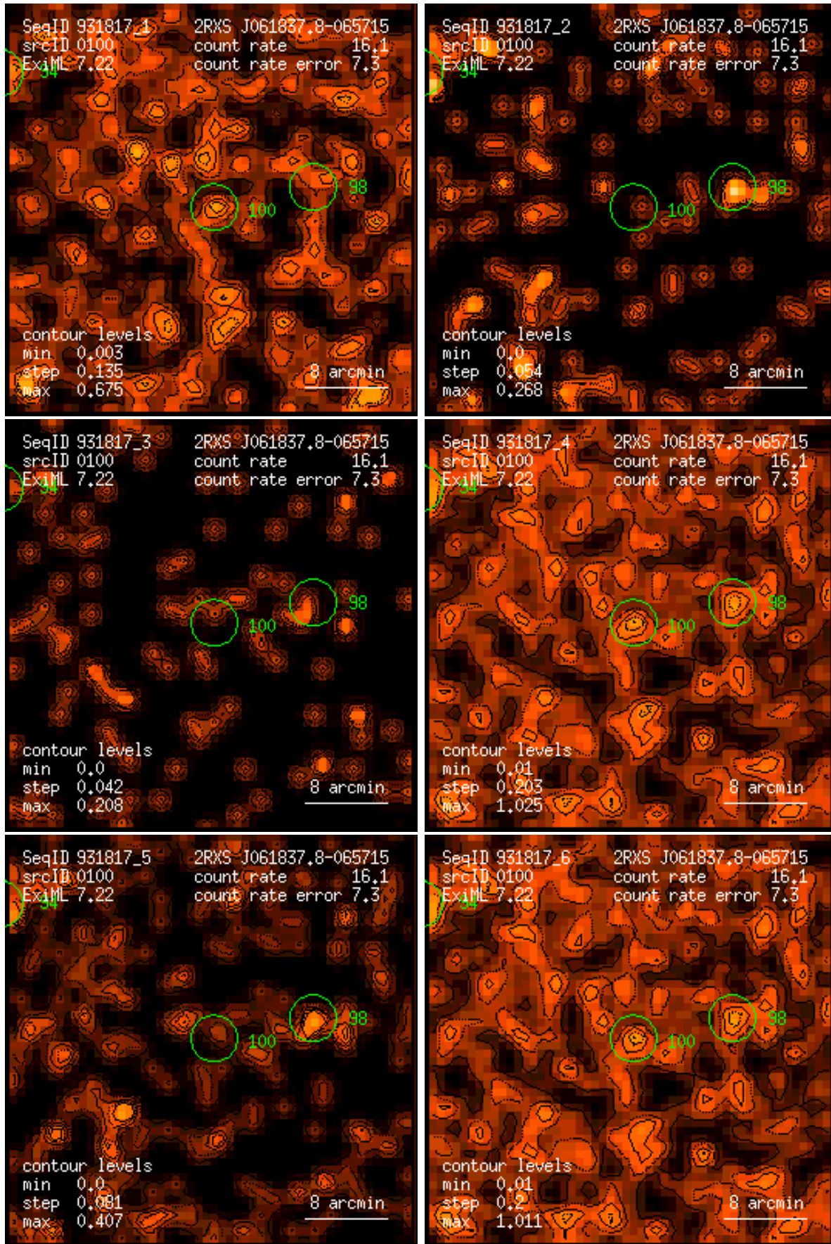
Figure 100: RASS 931817: detection 0100: band rate images, Gaussian filter: (1) PSPC channels 11 – 41, (2) 52 – 90, (3) 91 – 201, (4) 11 – 235, (5) 52 – 201, (6) 11 – 201. Broad band rates in counts/ks. Band rate contour levels in counts/ks/arcmin 2 .
