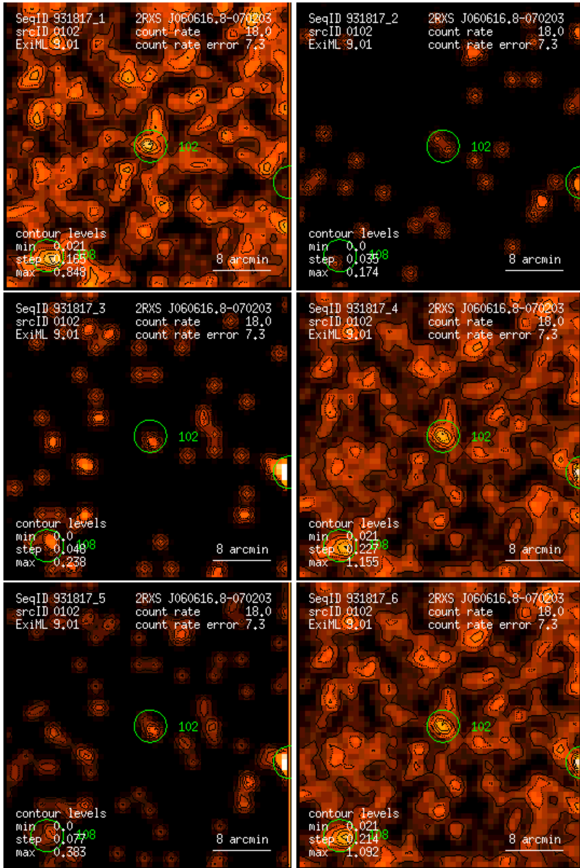
Figure 102: RASS 931817: detection 0102: band rate images, Gaussian filter: (1) PSPC channels 11 – 41, (2) 52 – 90, (3) 91 – 201, (4) 11 – 235, (5) 52 – 201, (6) 11 – 201. Broad band rates in counts/ks. Band rate contour levels in counts/ks/arcmin 2 .
