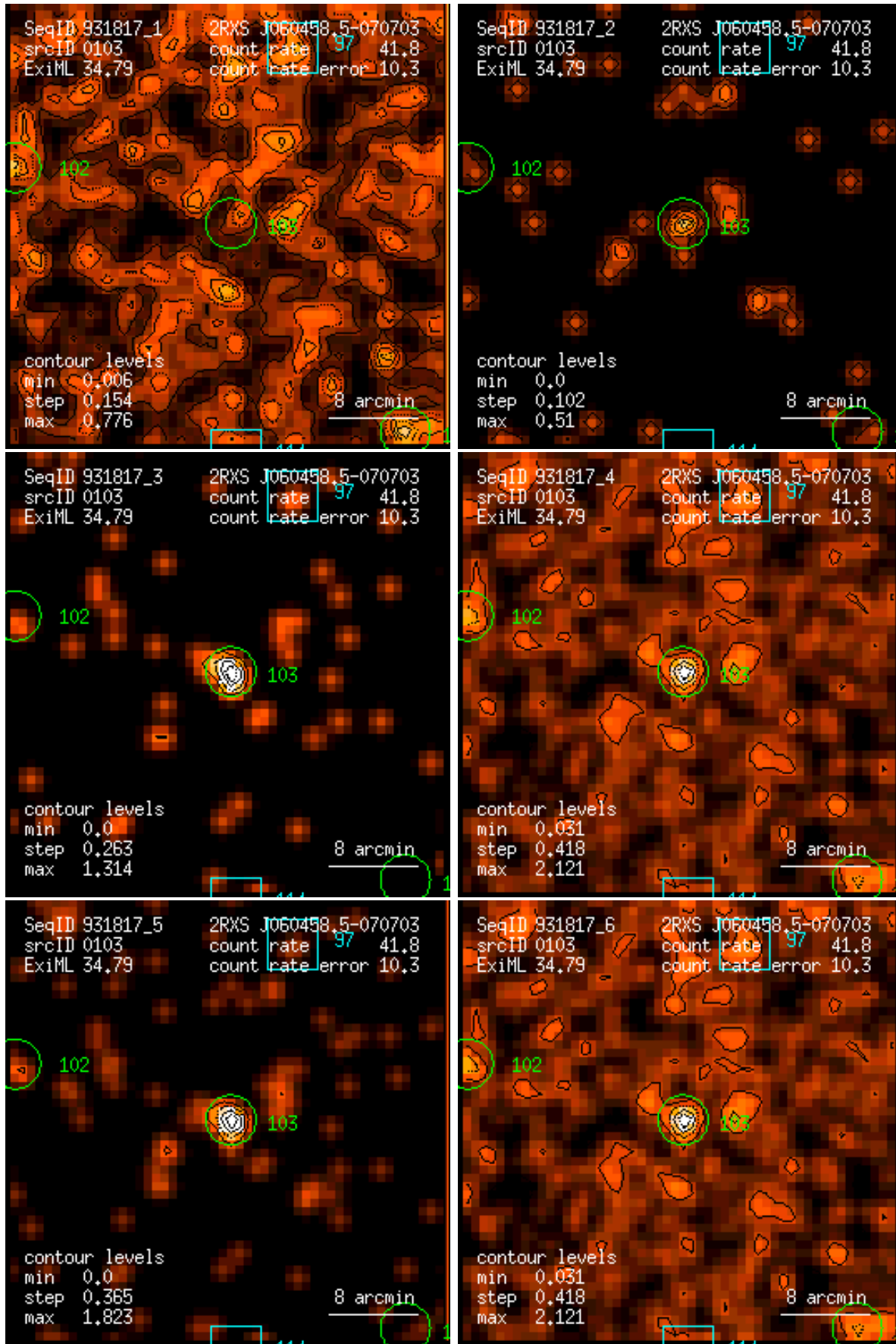
Figure 103: RASS 931817: detection 0103: band rate images, Gaussian filter: (1) PSPC channels 11 – 41, (2) 52 – 90, (3) 91 – 201, (4) 11 – 235, (5) 52 – 201, (6) 11 – 201. Broad band rates in counts/ks. Band rate contour levels in counts/ks/arcmin 2 .
