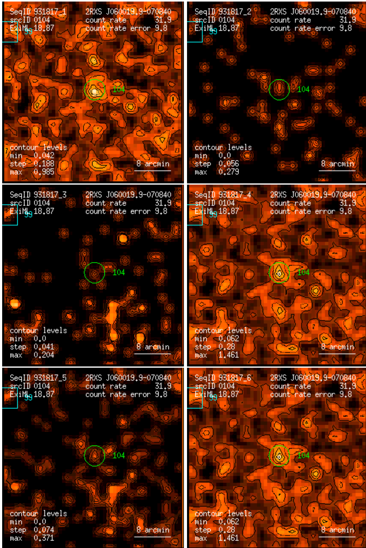
Figure 104: RASS 931817: detection 0104: band rate images, Gaussian filter: (1) PSPC channels 11 – 41, (2) 52 – 90, (3) 91 – 201, (4) 11 – 235, (5) 52 – 201, (6) 11 – 201. Broad band rates in counts/ks. Band rate contour levels in counts/ks/arcmin 2 .
