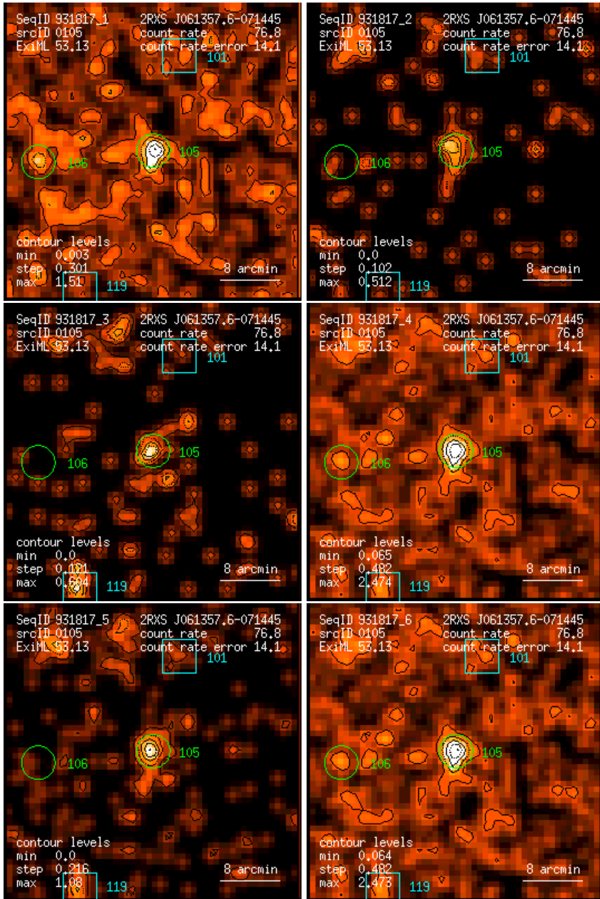
Figure 105: RASS 931817: detection 0105: band rate images, Gaussian filter: (1) PSPC channels 11 – 41, (2) 52 – 90, (3) 91 – 201, (4) 11 – 235, (5) 52 – 201, (6) 11 – 201. Broad band rates in counts/ks. Band rate contour levels in counts/ks/arcmin 2 .
