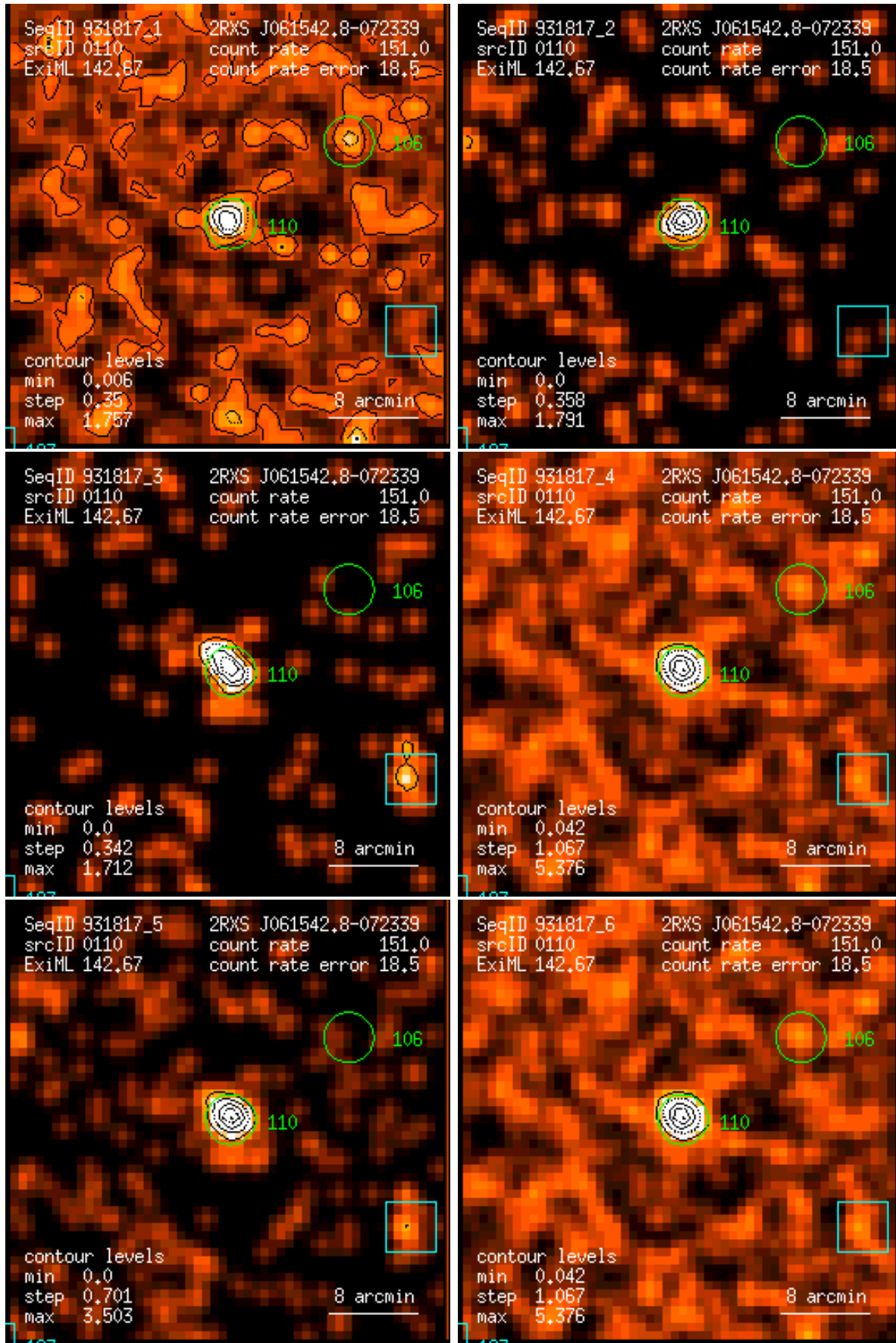
Figure 110: RASS 931817: detection 0110: band rate images, Gaussian filter: (1) PSPC channels 11 – 41, (2) 52 – 90, (3) 91 – 201, (4) 11 – 235, (5) 52 – 201, (6) 11 – 201. Broad band rates in counts/ks. Band rate contour levels in counts/ks/arcmin 2 .
