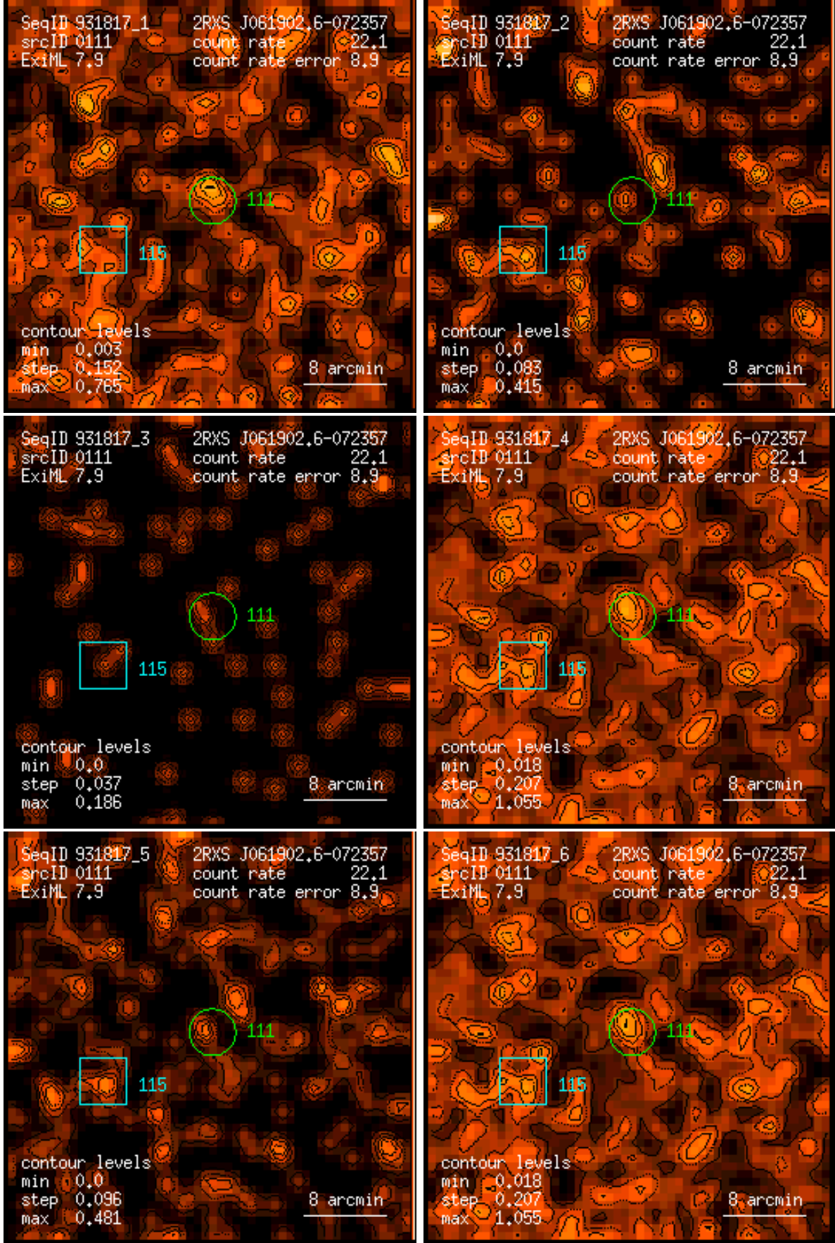
Figure 111: RASS 931817: detection 0111: band rate images, Gaussian filter: (1) PSPC channels 11 – 41, (2) 52 – 90, (3) 91 – 201, (4) 11 – 235, (5) 52 – 201, (6) 11 – 201. Broad band rates in counts/ks. Band rate contour levels in counts/ks/arcmin 2 .
