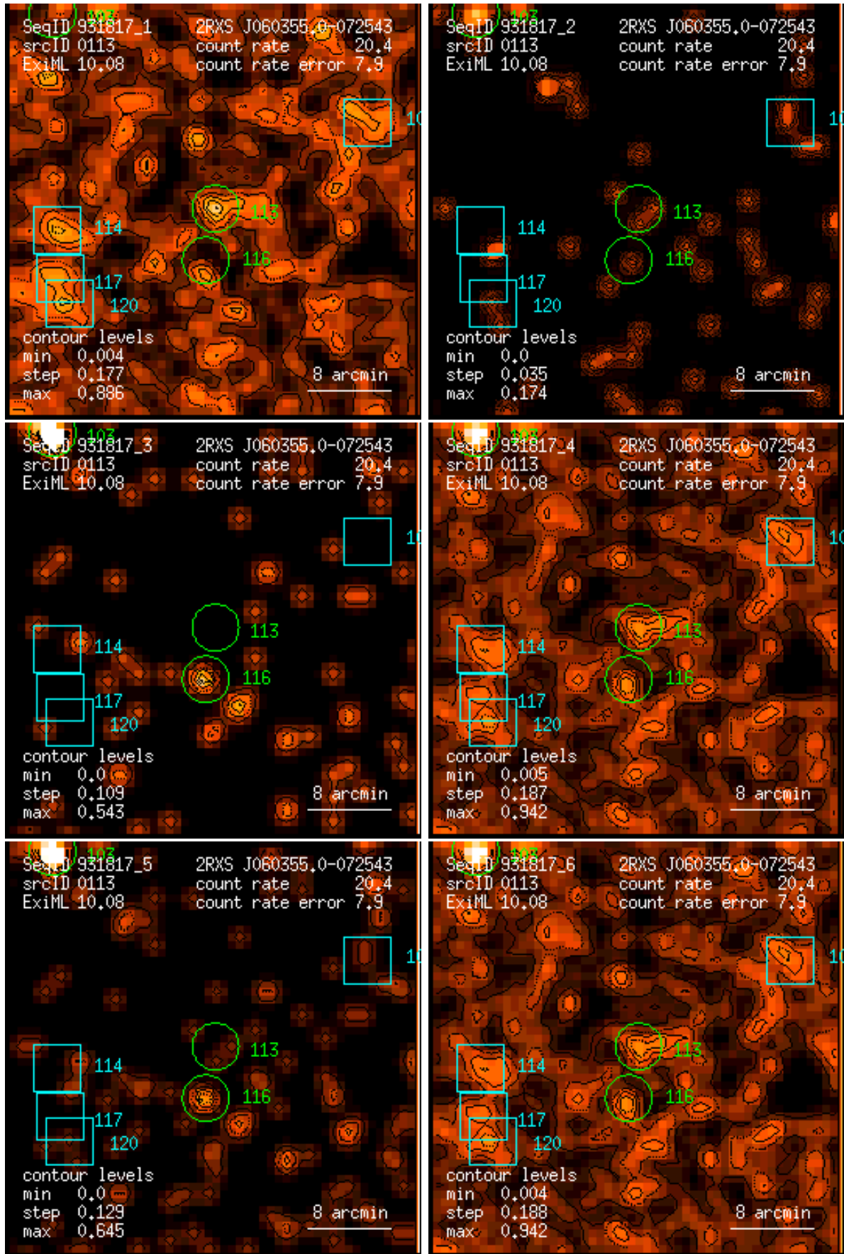
Figure 113: RASS 931817: detection 0113: band rate images, Gaussian filter: (1) PSPC channels 11 – 41, (2) 52 – 90, (3) 91 – 201, (4) 11 – 235, (5) 52 – 201, (6) 11 – 201. Broad band rates in counts/ks. Band rate contour levels in counts/ks/arcmin 2 .
