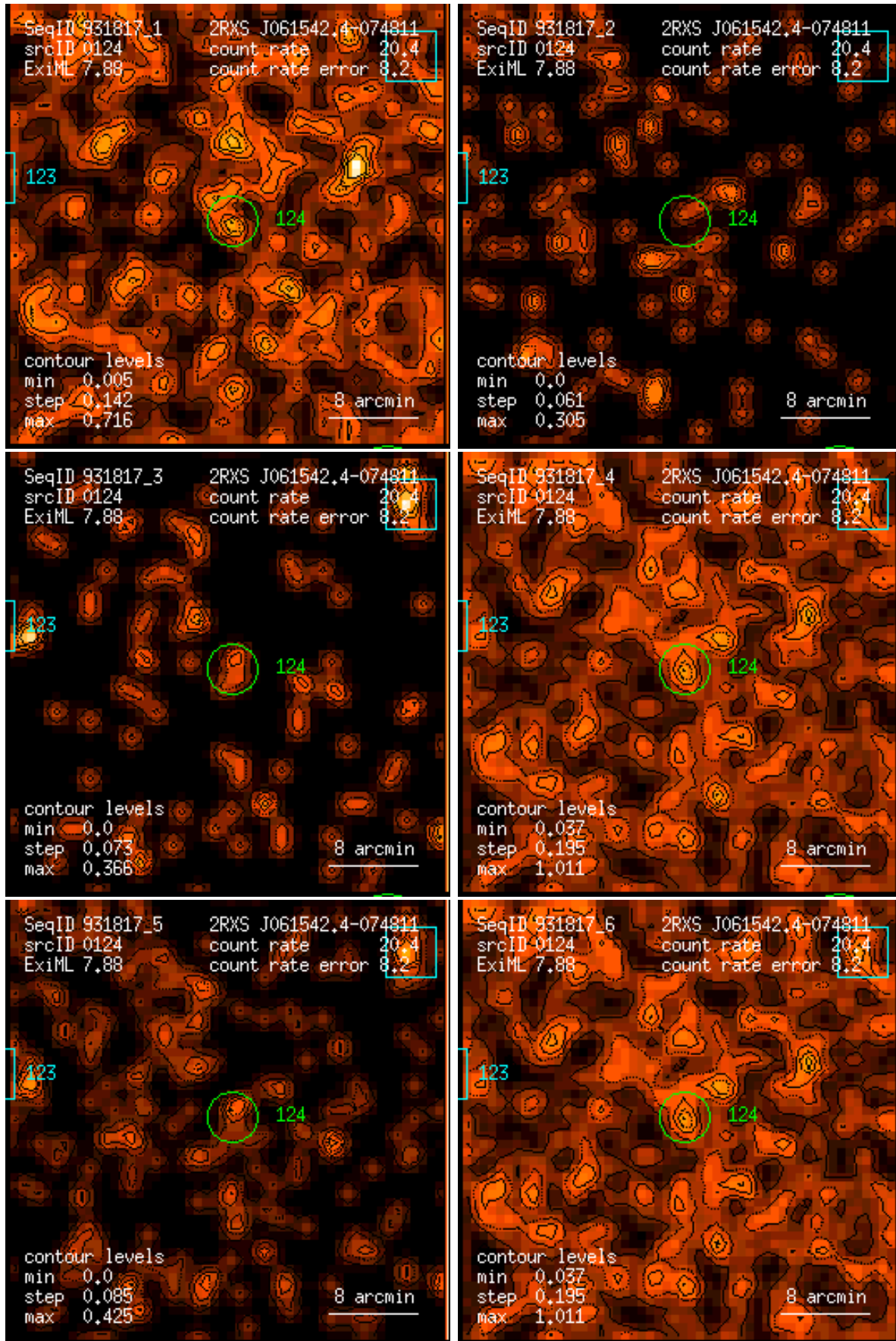
Figure 124: RASS 931817: detection 0124: band rate images, Gaussian filter: (1) PSPC channels 11 – 41, (2) 52 – 90, (3) 91 – 201, (4) 11 – 235, (5) 52 – 201, (6) 11 – 201. Broad band rates in counts/ks. Band rate contour levels in counts/ks/arcmin 2 .
