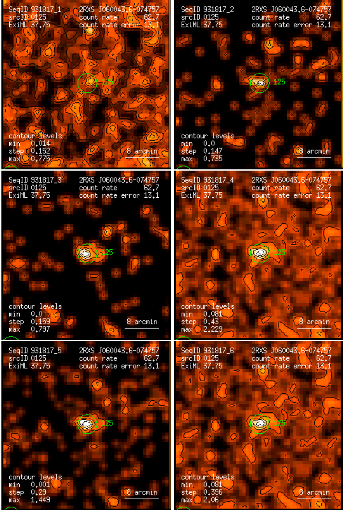
Figure 125: RASS 931817: detection 0125: band rate images, Gaussian filter: (1) PSPC channels 11 – 41, (2) 52 – 90, (3) 91 – 201, (4) 11 – 235, (5) 52 – 201, (6) 11 – 201. Broad band rates in counts/ks. Band rate contour levels in counts/ks/arcmin 2 .
