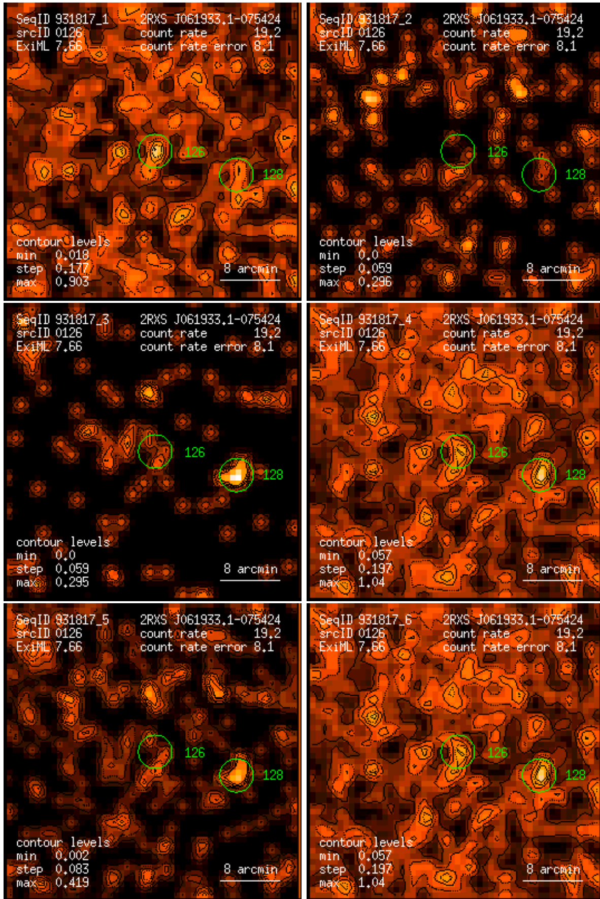
Figure 126: RASS 931817: detection 0126: band rate images, Gaussian filter: (1) PSPC channels 11 – 41, (2) 52 – 90, (3) 91 – 201, (4) 11 – 235, (5) 52 – 201, (6) 11 – 201. Broad band rates in counts/ks. Band rate contour levels in counts/ks/arcmin 2 .
