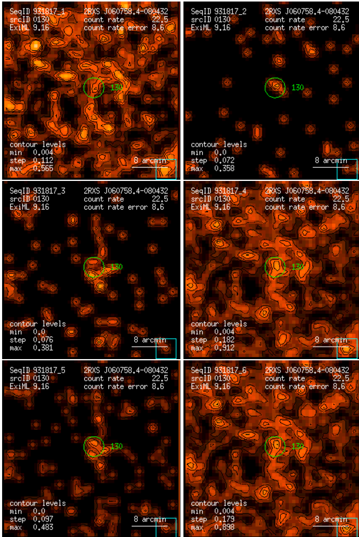
Figure 130: RASS 931817: detection 0130: band rate images, Gaussian filter: (1) PSPC channels 11 – 41, (2) 52 – 90, (3) 91 – 201, (4) 11 – 235, (5) 52 – 201, (6) 11 – 201. Broad band rates in counts/ks. Band rate contour levels in counts/ks/arcmin 2 .
