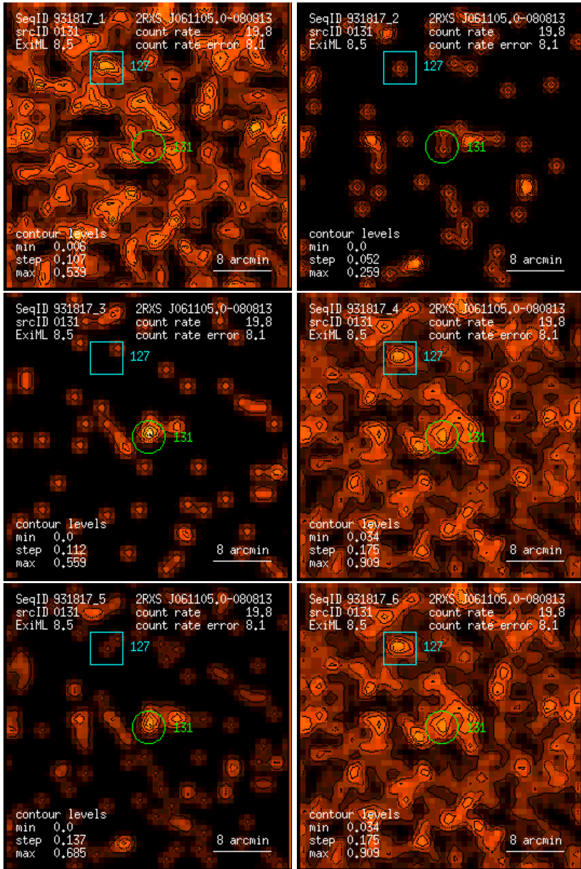
Figure 131: RASS 931817: detection 0131: band rate images, Gaussian filter: (1) PSPC channels 11 – 41, (2) 52 – 90, (3) 91 – 201, (4) 11 – 235, (5) 52 – 201, (6) 11 – 201. Broad band rates in counts/ks. Band rate contour levels in counts/ks/arcmin 2 .
