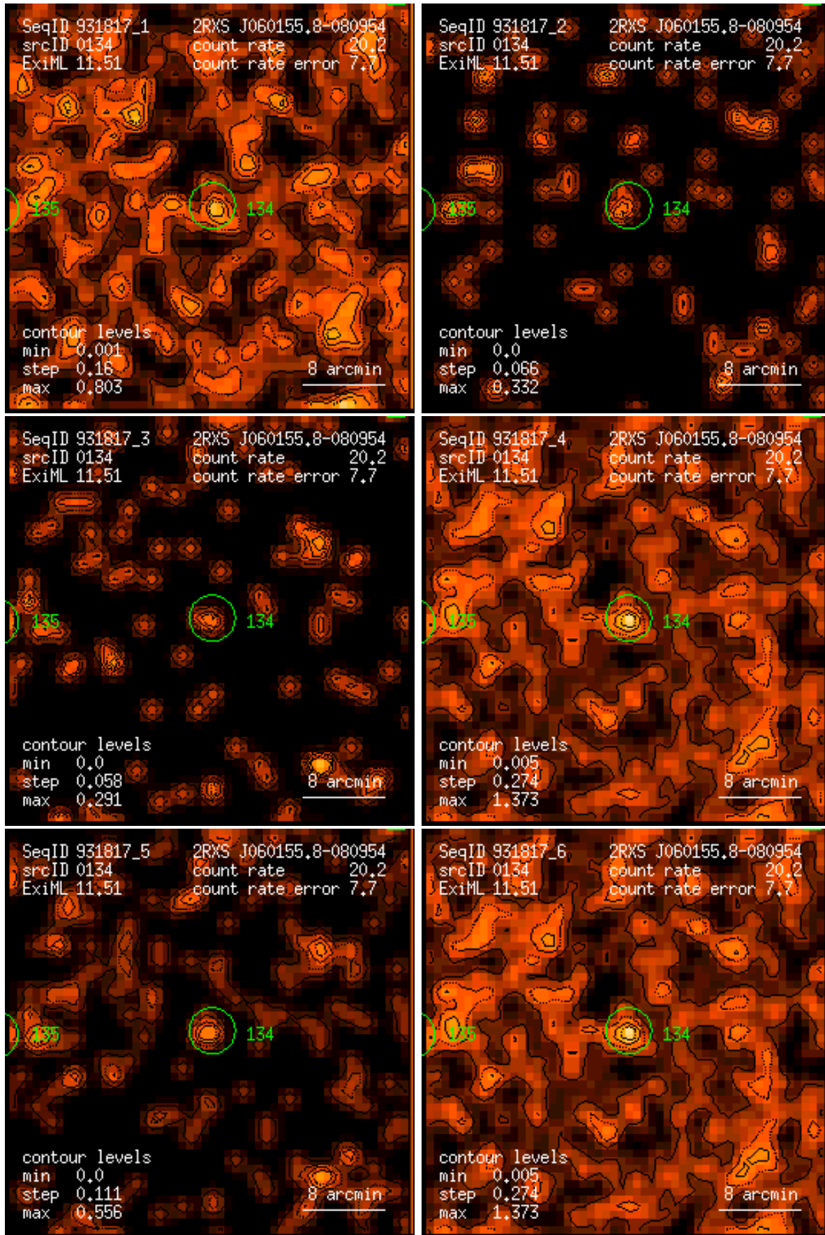
Figure 134: RASS 931817: detection 0134: band rate images, Gaussian filter: (1) PSPC channels 11 – 41, (2) 52 – 90, (3) 91 – 201, (4) 11 – 235, (5) 52 – 201, (6) 11 – 201. Broad band rates in counts/ks. Band rate contour levels in counts/ks/arcmin 2 .
