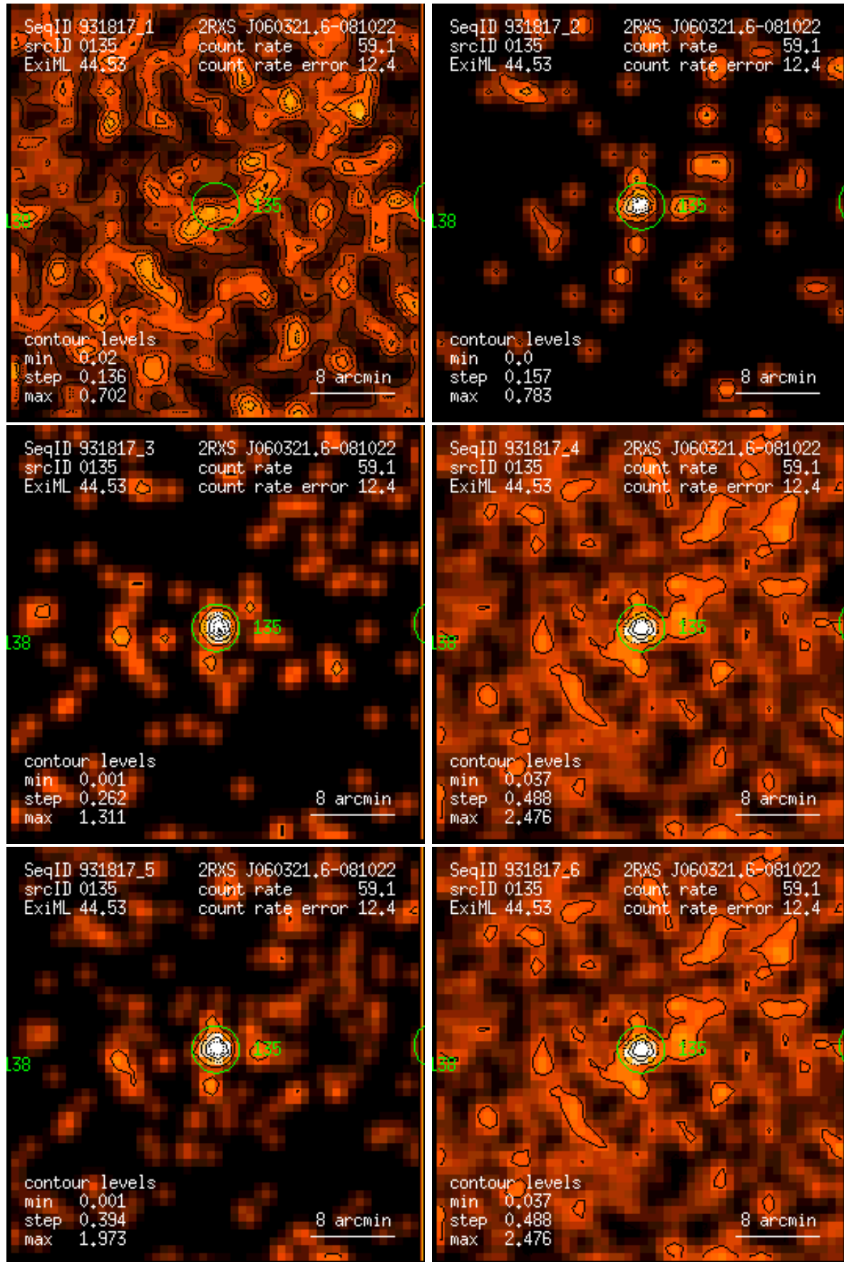
Figure 135: RASS 931817: detection 0135: band rate images, Gaussian filter: (1) PSPC channels 11 – 41, (2) 52 – 90, (3) 91 – 201, (4) 11 – 235, (5) 52 – 201, (6) 11 – 201. Broad band rates in counts/ks. Band rate contour levels in counts/ks/arcmin 2 .
