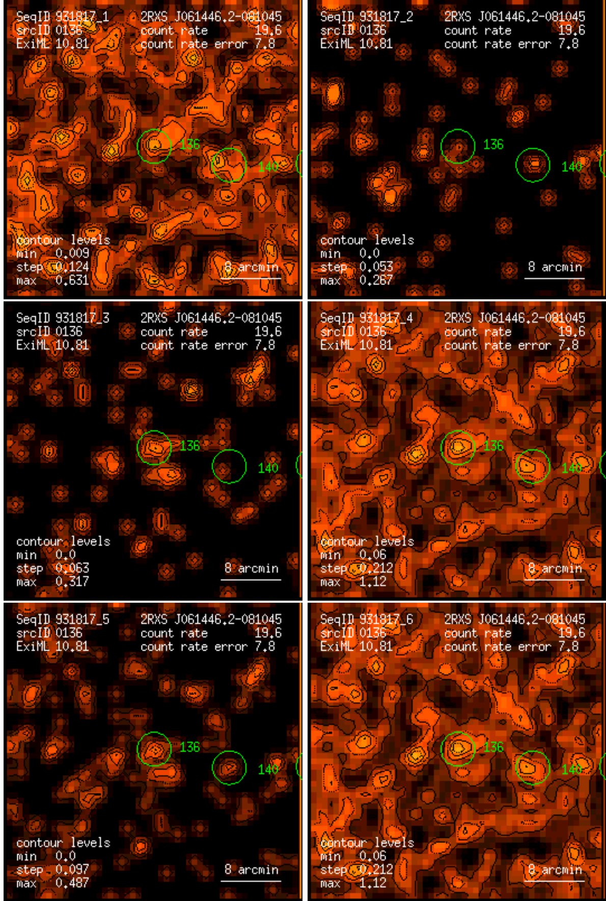
Figure 136: RASS 931817: detection 0136: band rate images, Gaussian filter: (1) PSPC channels 11 – 41, (2) 52 – 90, (3) 91 – 201, (4) 11 – 235, (5) 52 – 201, (6) 11 – 201. Broad band rates in counts/ks. Band rate contour levels in counts/ks/arcmin 2 .
