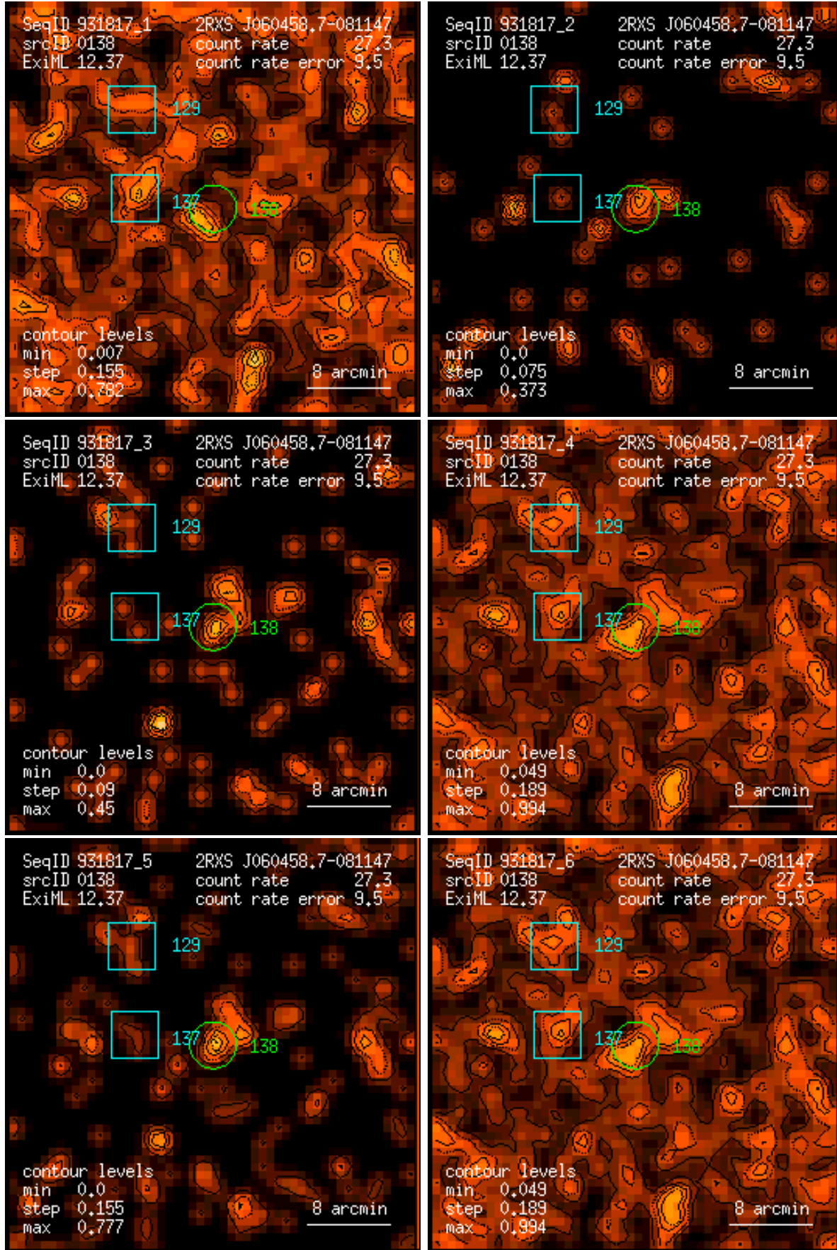
Figure 138: RASS 931817: detection 0138: band rate images, Gaussian filter: (1) PSPC channels 11 – 41, (2) 52 – 90, (3) 91 – 201, (4) 11 – 235, (5) 52 – 201, (6) 11 – 201. Broad band rates in counts/ks. Band rate contour levels in counts/ks/arcmin 2 .
