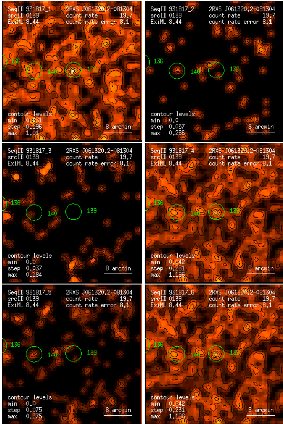
Figure 139: RASS 931817: detection 0139: band rate images, Gaussian filter: (1) PSPC channels 11 – 41, (2) 52 – 90, (3) 91 – 201, (4) 11 – 235, (5) 52 – 201, (6) 11 – 201. Broad band rates in counts/ks. Band rate contour levels in counts/ks/arcmin 2 .
