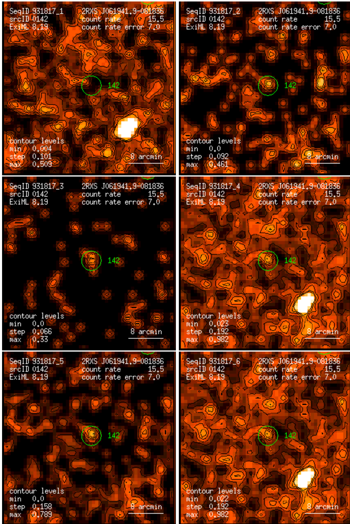
Figure 142: RASS 931817: detection 0142: band rate images, Gaussian filter: (1) PSPC channels 11 – 41, (2) 52 – 90, (3) 91 – 201, (4) 11 – 235, (5) 52 – 201, (6) 11 – 201. Broad band rates in counts/ks. Band rate contour levels in counts/ks/arcmin 2 .
