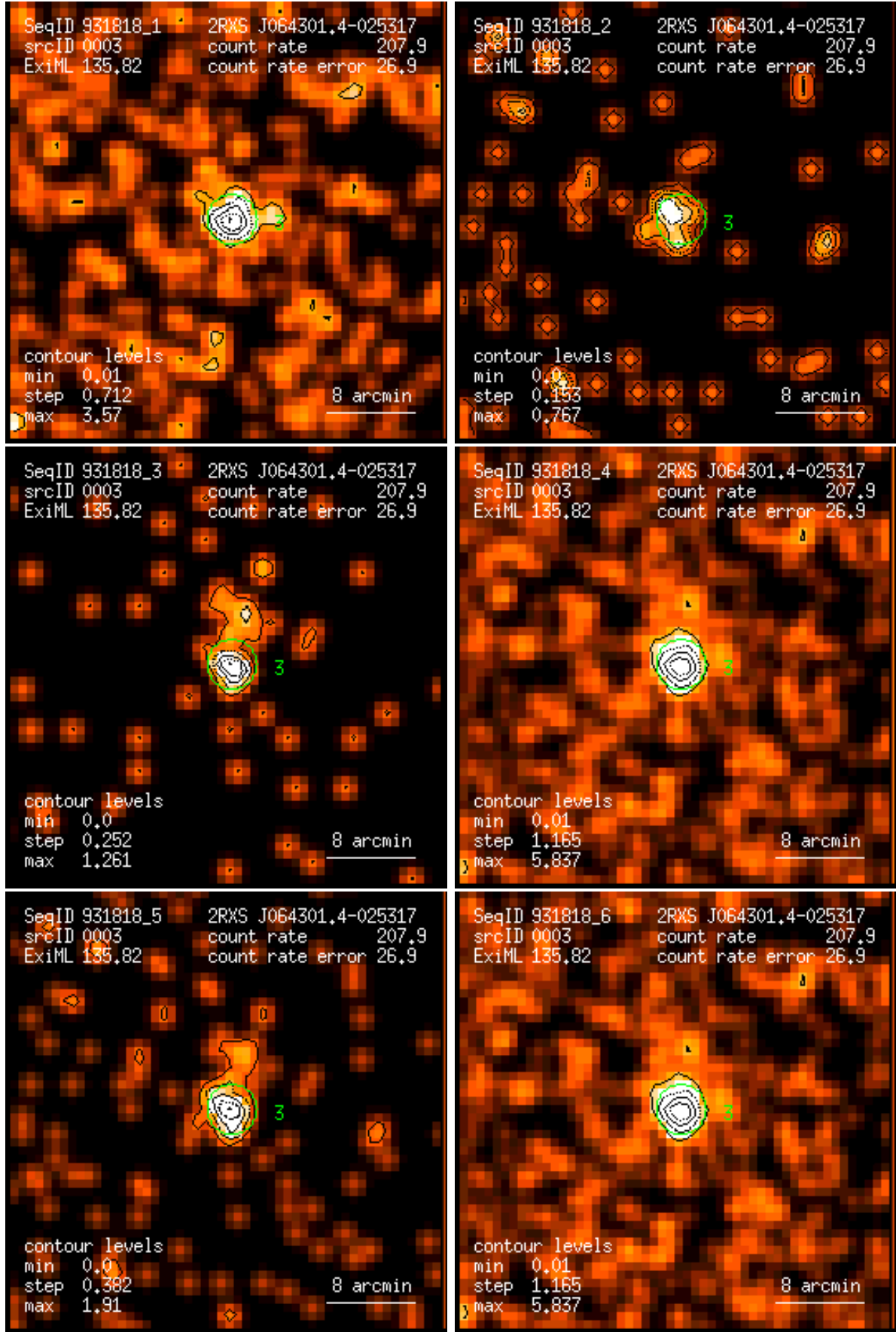
Figure 3: RASS 931818: detection 0003: band rate images, Gaussian filter: (1) PSPC channels 11 – 41, (2) 52 – 90, (3) 91 – 201, (4) 11 – 235, (5) 52 – 201, (6) 11 – 201. Broad band rates in counts/ks. Band rate contour levels in counts/ks/arcmin 2 .
