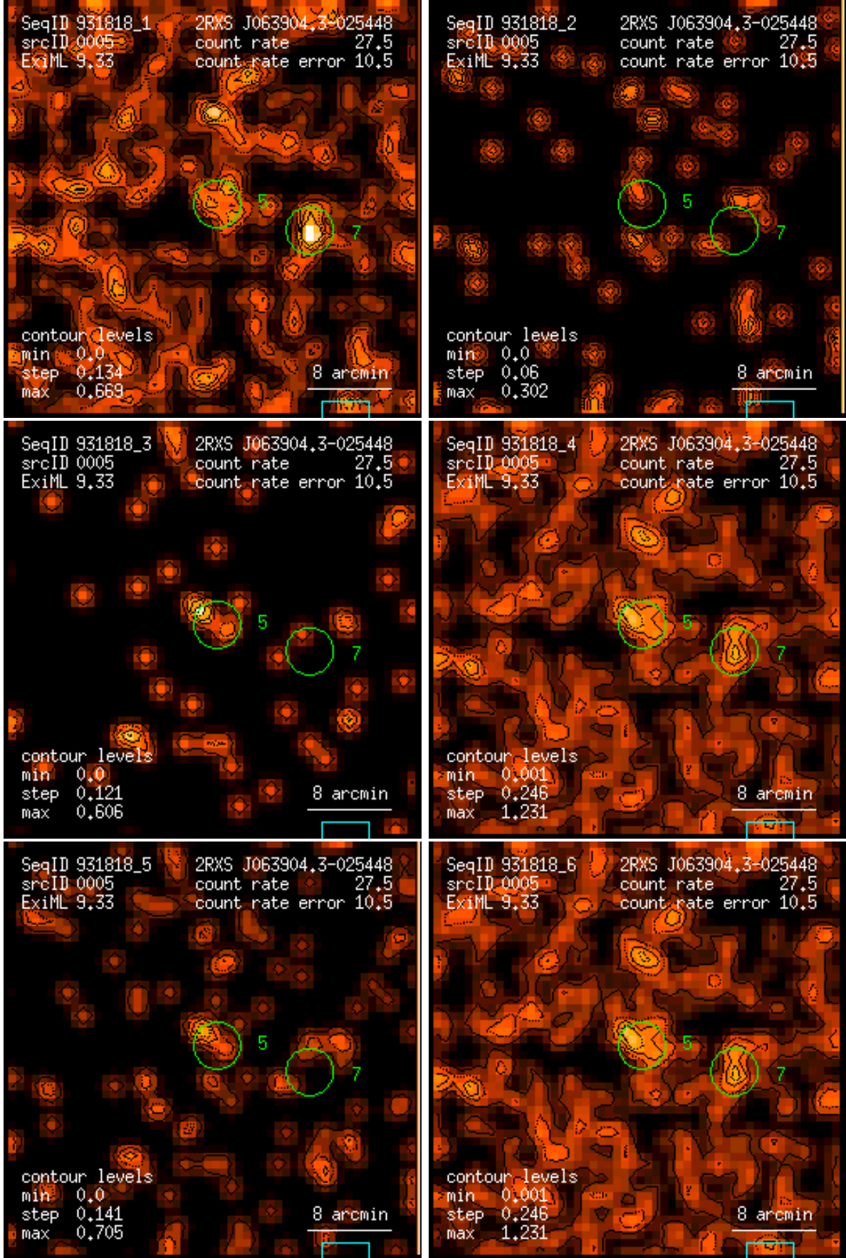
Figure 5: RASS 931818: detection 0005: band rate images, Gaussian filter: (1) PSPC channels 11 – 41, (2) 52 – 90, (3) 91 – 201, (4) 11 – 235, (5) 52 – 201, (6) 11 – 201. Broad band rates in counts/ks. Band rate contour levels in counts/ks/arcmin 2 .
