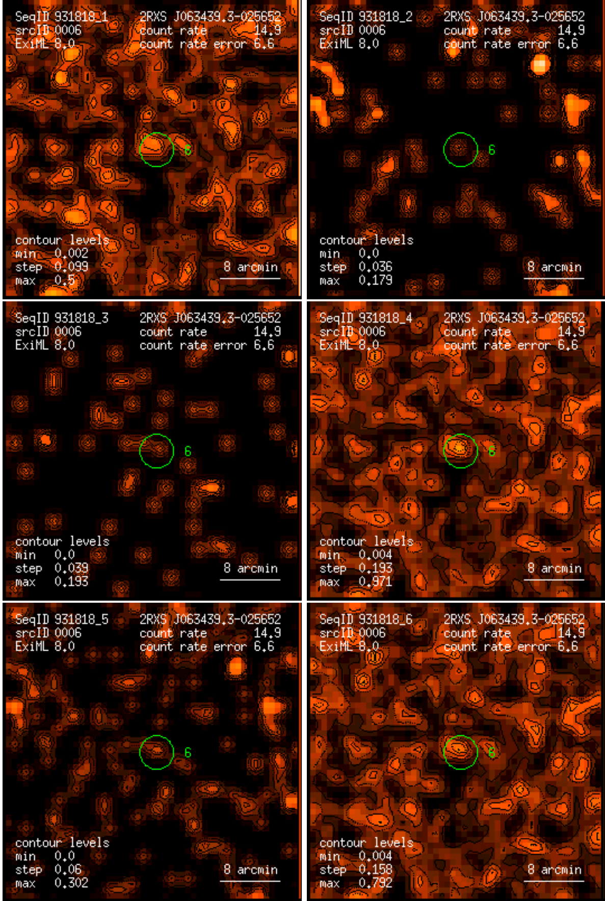
Figure 6: RASS 931818: detection 0006: band rate images, Gaussian filter: (1) PSPC channels 11 – 41, (2) 52 – 90, (3) 91 – 201, (4) 11 – 235, (5) 52 – 201, (6) 11 – 201. Broad band rates in counts/ks. Band rate contour levels in counts/ks/arcmin 2 .
