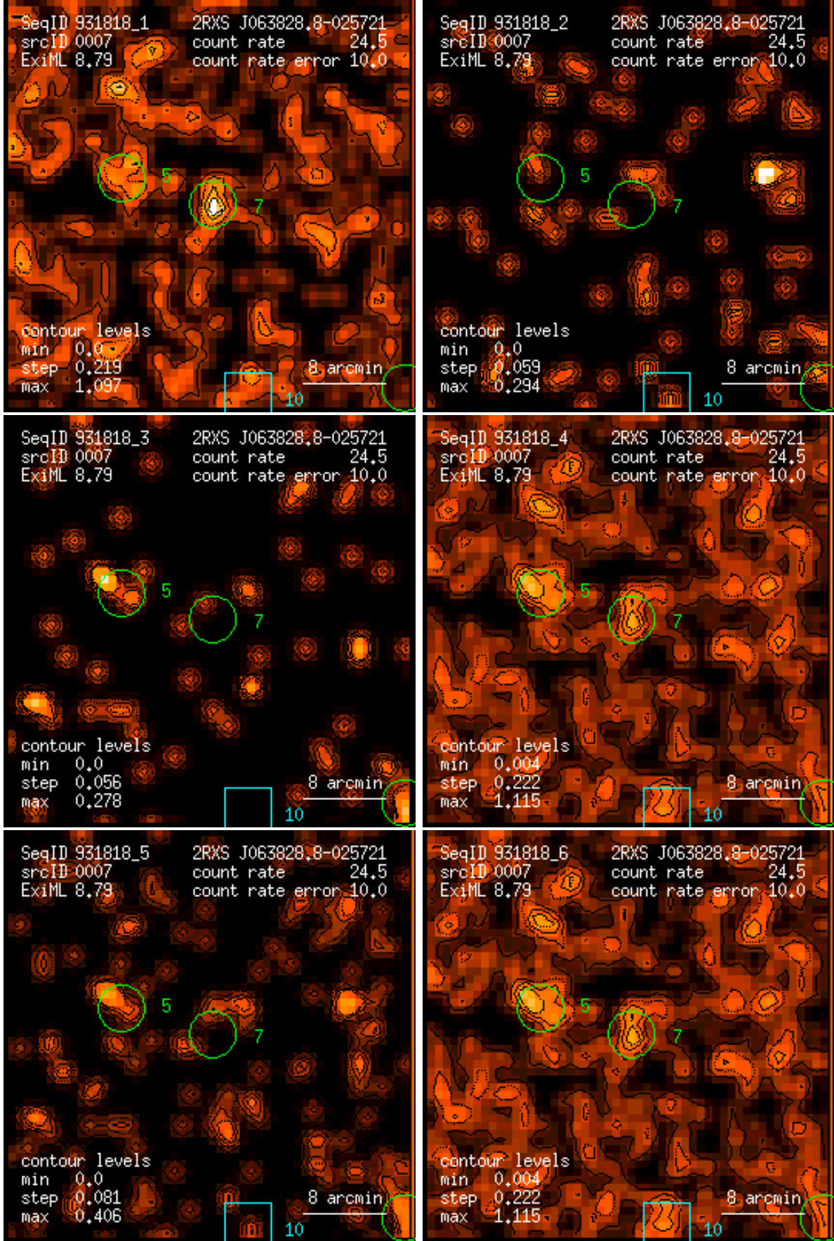
Figure 7: RASS 931818: detection 0007: band rate images, Gaussian filter: (1) PSPC channels 11 – 41, (2) 52 – 90, (3) 91 – 201, (4) 11 – 235, (5) 52 – 201, (6) 11 – 201. Broad band rates in counts/ks. Band rate contour levels in counts/ks/arcmin 2 .
