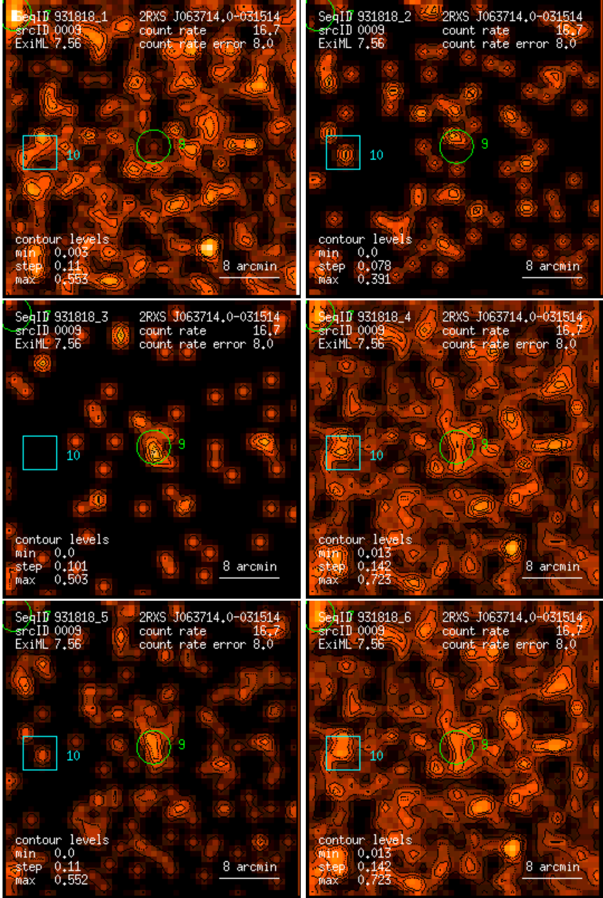
Figure 9: RASS 931818: detection 0009: band rate images, Gaussian filter: (1) PSPC channels 11 – 41, (2) 52 – 90, (3) 91 – 201, (4) 11 – 235, (5) 52 – 201, (6) 11 – 201. Broad band rates in counts/ks. Band rate contour levels in counts/ks/arcmin 2 .
