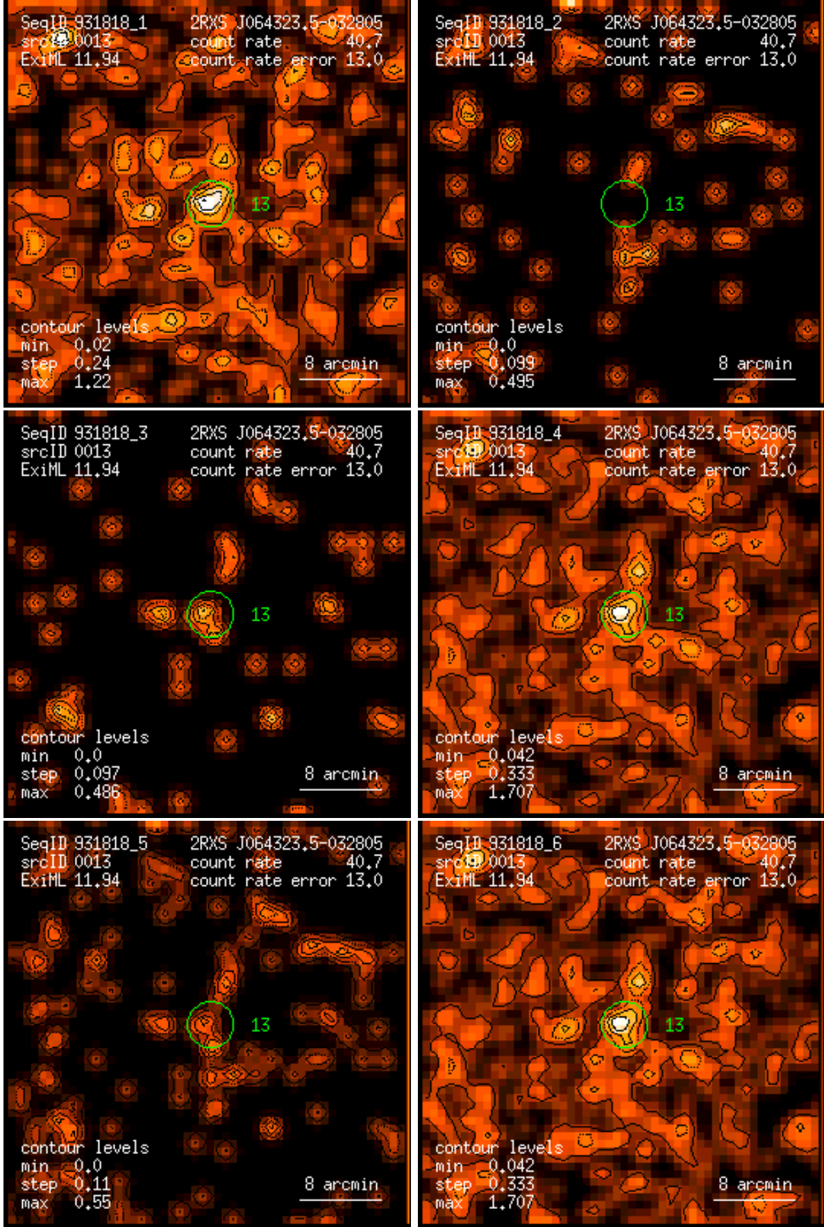
Figure 13: RASS 931818: detection 0013: band rate images, Gaussian filter: (1) PSPC channels 11 – 41, (2) 52 – 90, (3) 91 – 201, (4) 11 – 235, (5) 52 – 201, (6) 11 – 201. Broad band rates in counts/ks. Band rate contour levels in counts/ks/arcmin 2 .
