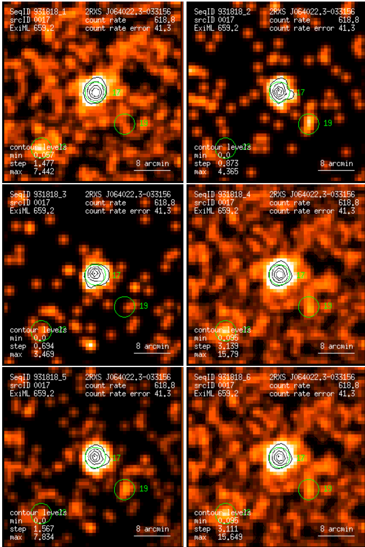
Figure 17: RASS 931818: detection 0017: band rate images, Gaussian filter: (1) PSPC channels 11 – 41, (2) 52 – 90, (3) 91 – 201, (4) 11 – 235, (5) 52 – 201, (6) 11 – 201. Broad band rates in counts/ks. Band rate contour levels in counts/ks/arcmin 2 .
