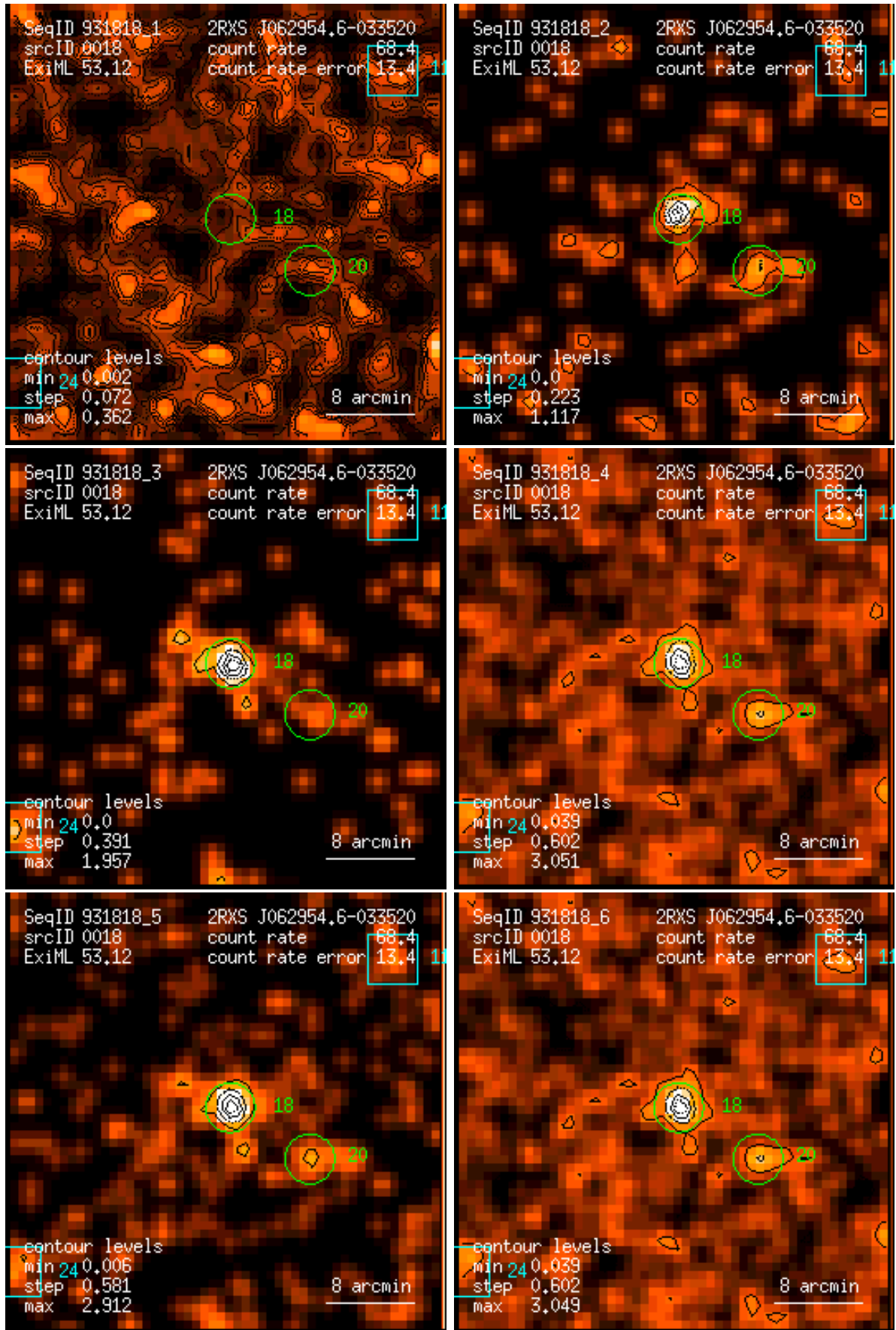
Figure 18: RASS 931818: detection 0018: band rate images, Gaussian filter: (1) PSPC channels 11 – 41, (2) 52 – 90, (3) 91 – 201, (4) 11 – 235, (5) 52 – 201, (6) 11 – 201. Broad band rates in counts/ks. Band rate contour levels in counts/ks/arcmin 2 .
