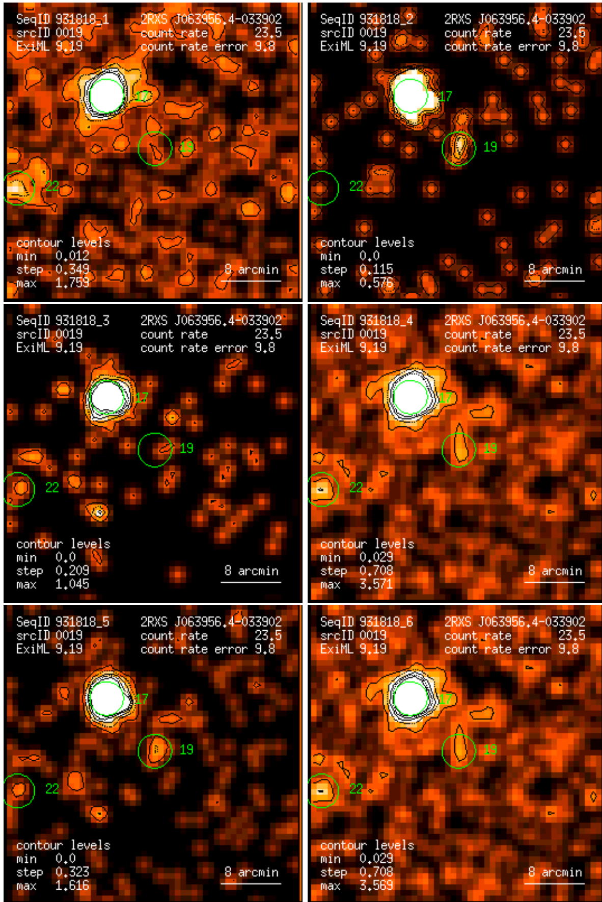
Figure 19: RASS 931818: detection 0019: band rate images, Gaussian filter: (1) PSPC channels 11 – 41, (2) 52 – 90, (3) 91 – 201, (4) 11 – 235, (5) 52 – 201, (6) 11 – 201. Broad band rates in counts/ks. Band rate contour levels in counts/ks/arcmin 2 .
