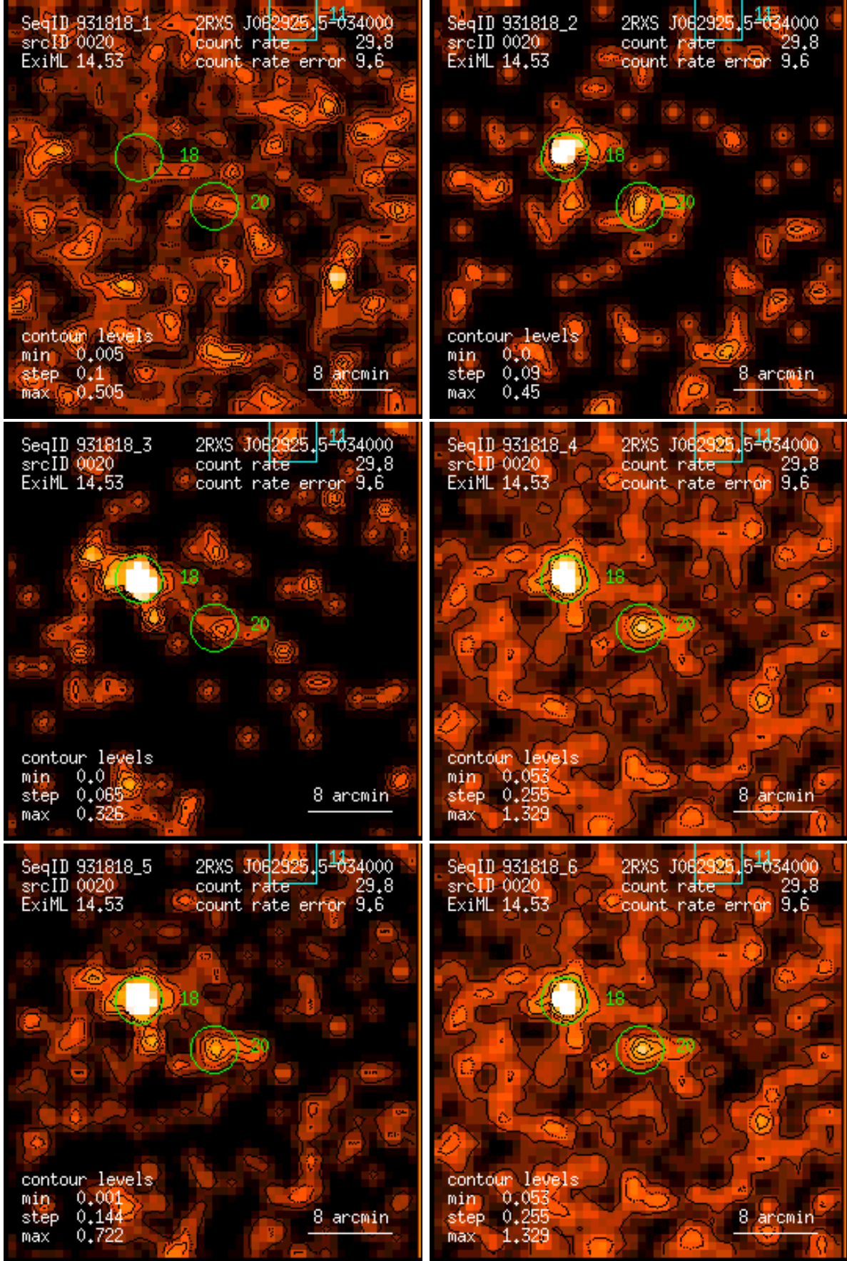
Figure 20: RASS 931818: detection 0020: band rate images, Gaussian filter: (1) PSPC channels 11 – 41, (2) 52 – 90, (3) 91 – 201, (4) 11 – 235, (5) 52 – 201, (6) 11 – 201. Broad band rates in counts/ks. Band rate contour levels in counts/ks/arcmin 2 .
