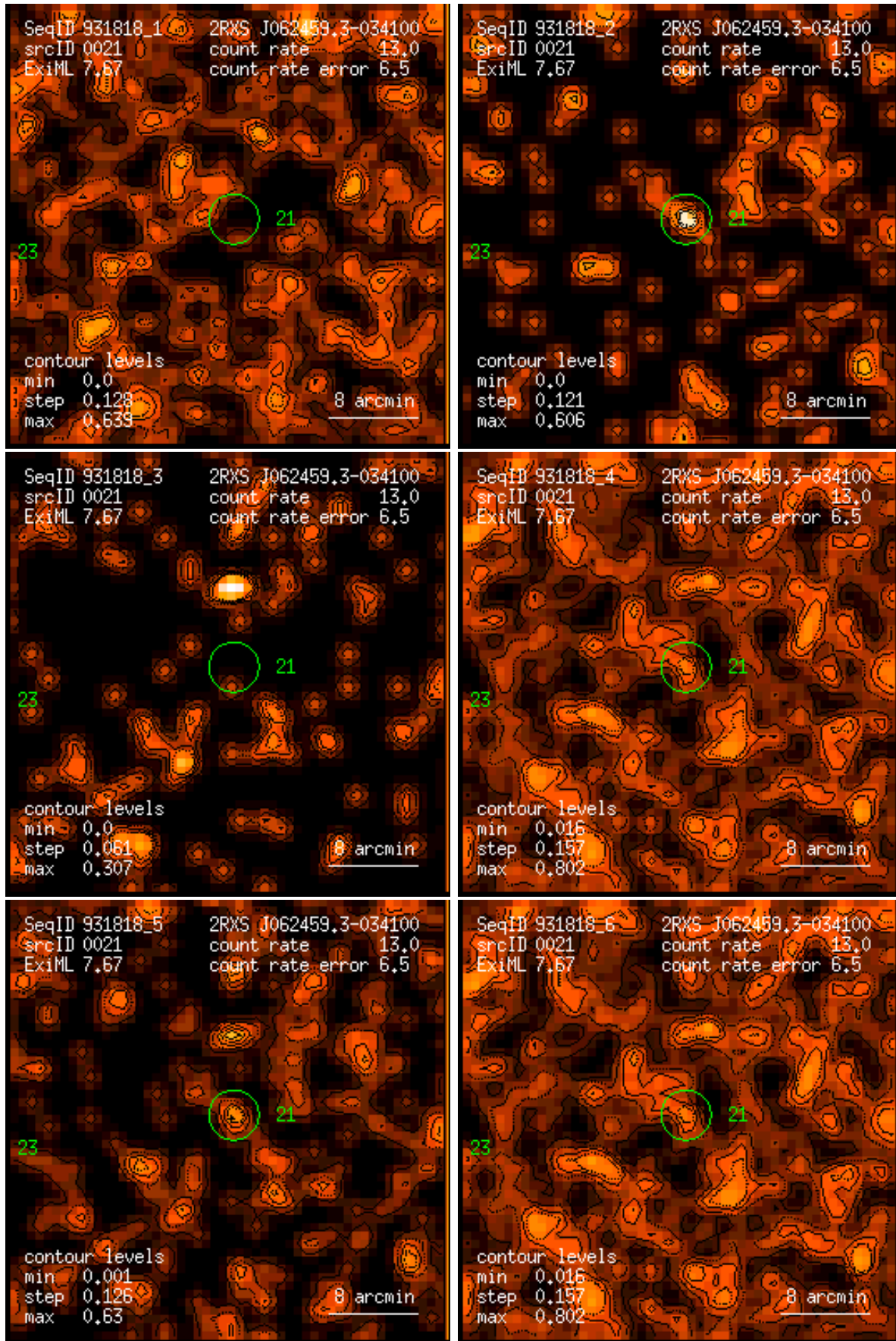
Figure 21: RASS 931818: detection 0021: band rate images, Gaussian filter: (1) PSPC channels 11 – 41, (2) 52 – 90, (3) 91 – 201, (4) 11 – 235, (5) 52 – 201, (6) 11 – 201. Broad band rates in counts/ks. Band rate contour levels in counts/ks/arcmin 2 .
