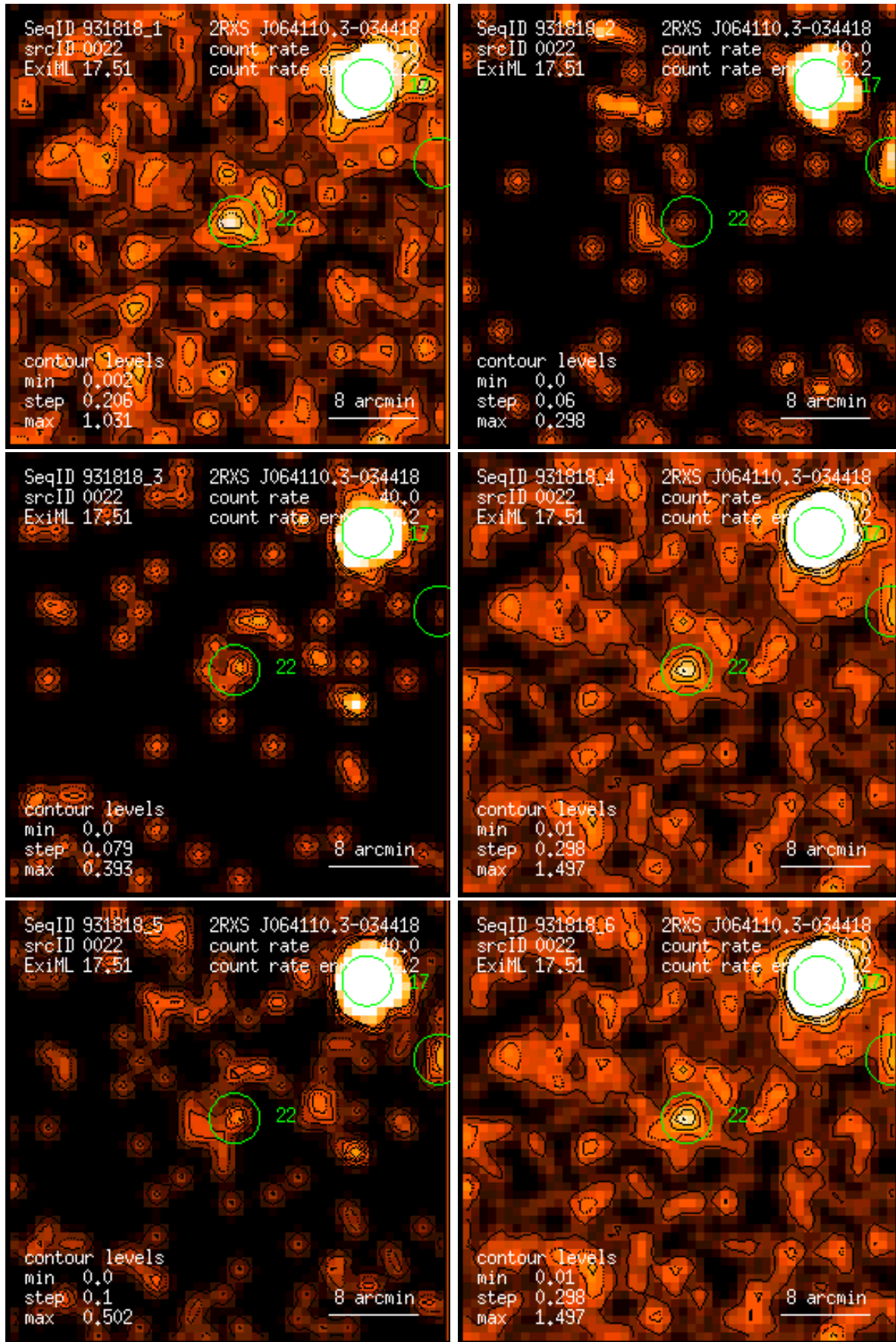
Figure 22: RASS 931818: detection 0022: band rate images, Gaussian filter: (1) PSPC channels 11 – 41, (2) 52 – 90, (3) 91 – 201, (4) 11 – 235, (5) 52 – 201, (6) 11 – 201. Broad band rates in counts/ks. Band rate contour levels in counts/ks/arcmin 2 .
