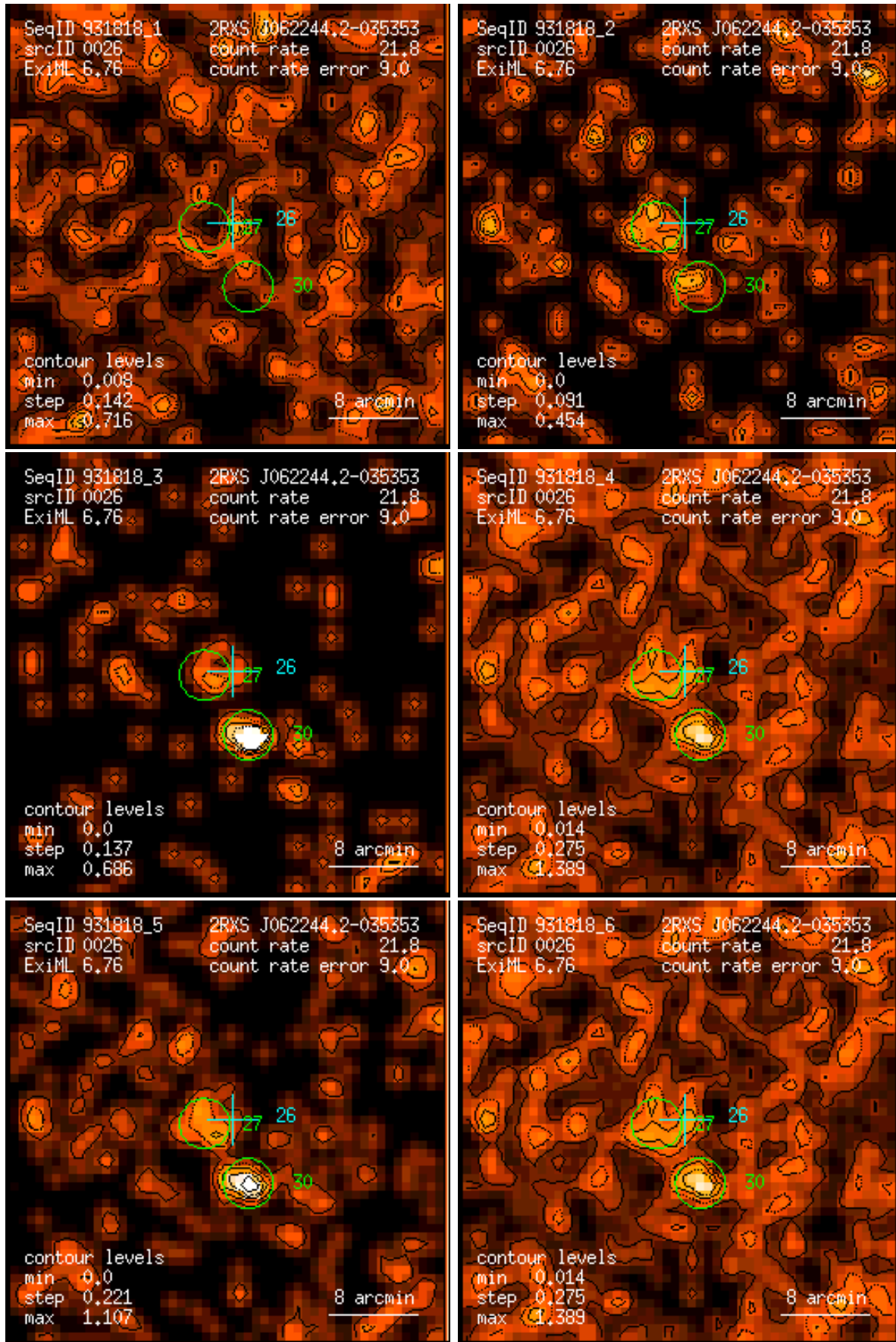
Figure 26: RASS 931818: detection 0026: band rate images, Gaussian filter: (1) PSPC channels 11 – 41, (2) 52 – 90, (3) 91 – 201, (4) 11 – 235, (5) 52 – 201, (6) 11 – 201. Broad band rates in counts/ks. Band rate contour levels in counts/ks/arcmin 2 .
