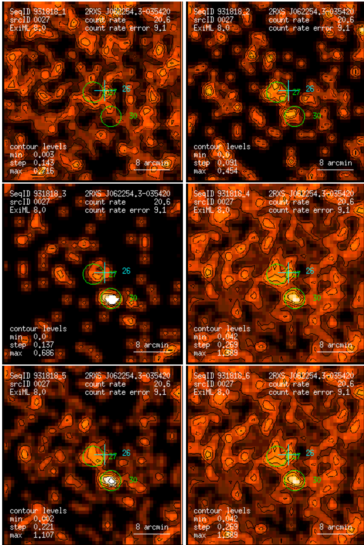
Figure 27: RASS 931818: detection 0027: band rate images, Gaussian filter: (1) PSPC channels 11 – 41, (2) 52 – 90, (3) 91 – 201, (4) 11 – 235, (5) 52 – 201, (6) 11 – 201. Broad band rates in counts/ks. Band rate contour levels in counts/ks/arcmin 2 .
