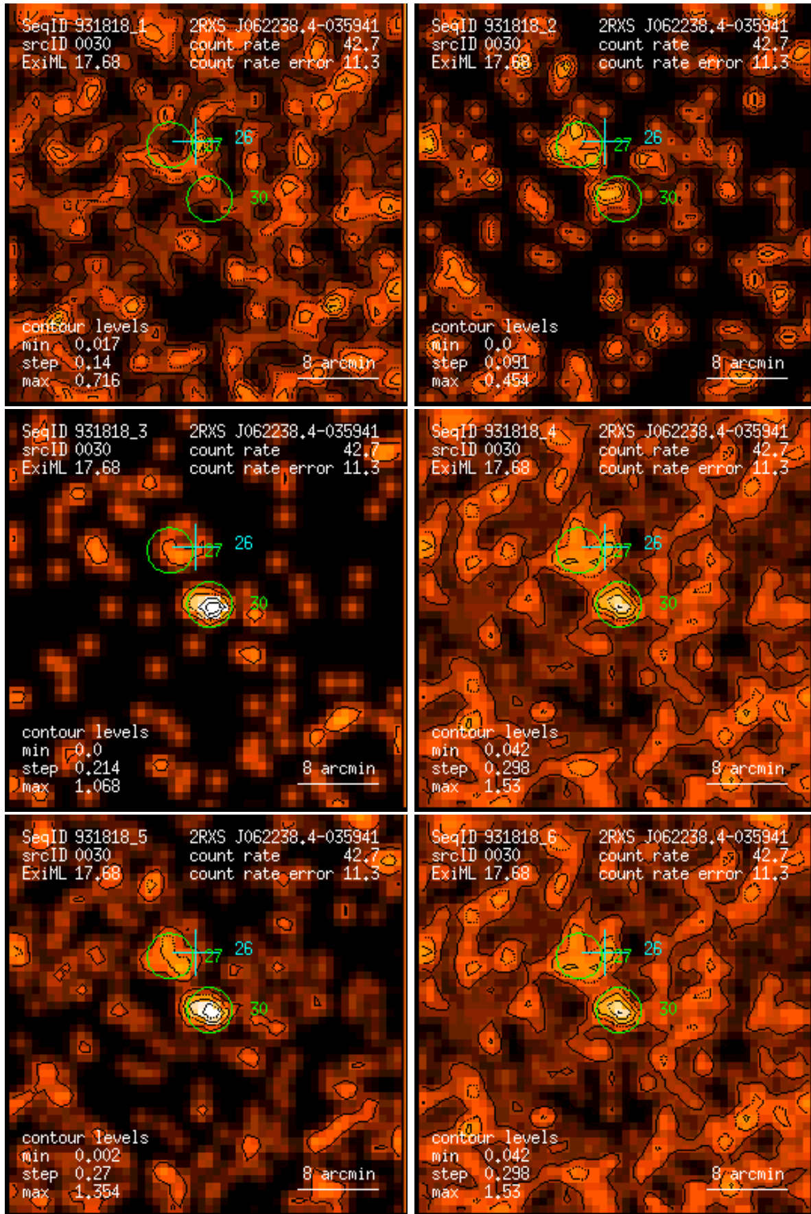
Figure 30: RASS 931818: detection 0030: band rate images, Gaussian filter: (1) PSPC channels 11 – 41, (2) 52 – 90, (3) 91 – 201, (4) 11 – 235, (5) 52 – 201, (6) 11 – 201. Broad band rates in counts/ks. Band rate contour levels in counts/ks/arcmin 2 .
