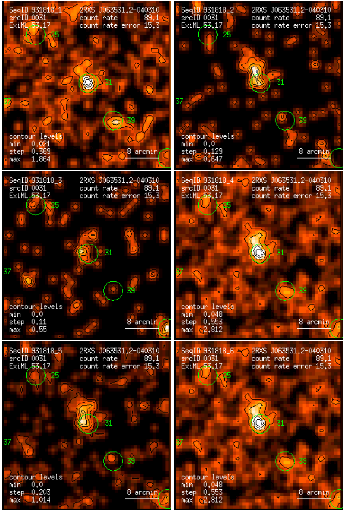
Figure 31: RASS 931818: detection 0031: band rate images, Gaussian filter: (1) PSPC channels 11 – 41, (2) 52 – 90, (3) 91 – 201, (4) 11 – 235, (5) 52 – 201, (6) 11 – 201. Broad band rates in counts/ks. Band rate contour levels in counts/ks/arcmin 2 .
