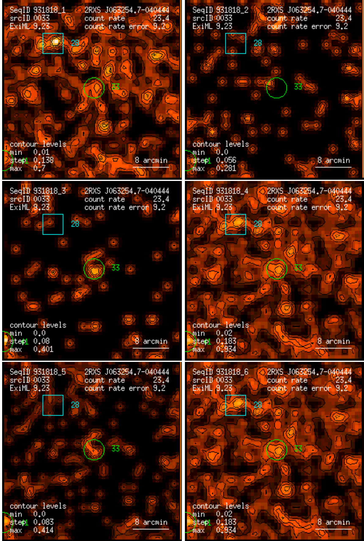
Figure 33: RASS 931818: detection 0033: band rate images, Gaussian filter: (1) PSPC channels 11 – 41, (2) 52 – 90, (3) 91 – 201, (4) 11 – 235, (5) 52 – 201, (6) 11 – 201. Broad band rates in counts/ks. Band rate contour levels in counts/ks/arcmin 2 .
