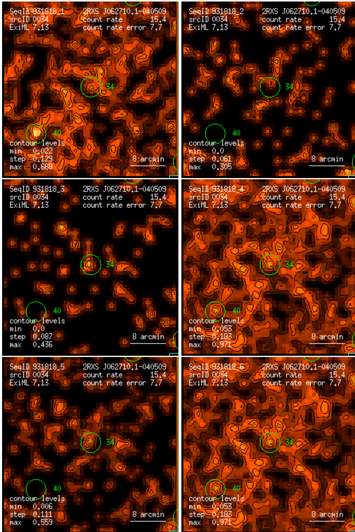
Figure 34: RASS 931818: detection 0034: band rate images, Gaussian filter: (1) PSPC channels 11 – 41, (2) 52 – 90, (3) 91 – 201, (4) 11 – 235, (5) 52 – 201, (6) 11 – 201. Broad band rates in counts/ks. Band rate contour levels in counts/ks/arcmin 2 .
