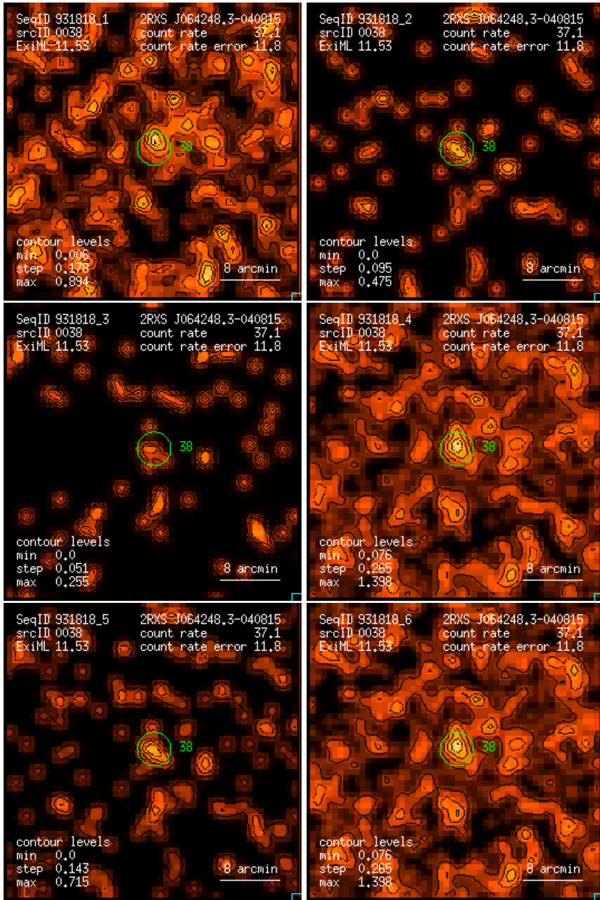
Figure 38: RASS 931818: detection 0038: band rate images, Gaussian filter: (1) PSPC channels 11 – 41, (2) 52 – 90, (3) 91 – 201, (4) 11 – 235, (5) 52 – 201, (6) 11 – 201. Broad band rates in counts/ks. Band rate contour levels in counts/ks/arcmin 2 .
