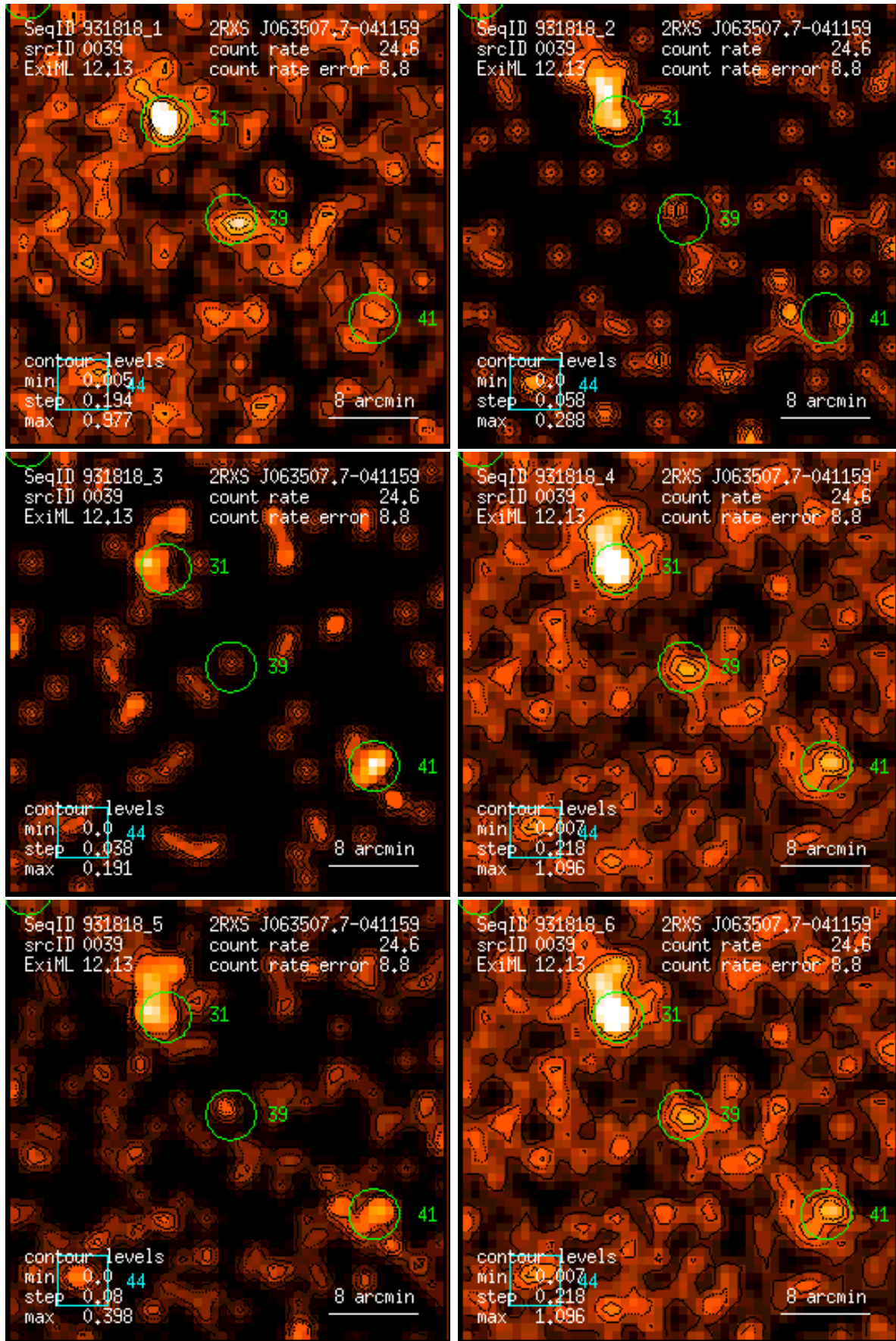
Figure 39: RASS 931818: detection 0039: band rate images, Gaussian filter: (1) PSPC channels 11 – 41, (2) 52 – 90, (3) 91 – 201, (4) 11 – 235, (5) 52 – 201, (6) 11 – 201. Broad band rates in counts/ks. Band rate contour levels in counts/ks/arcmin 2 .
