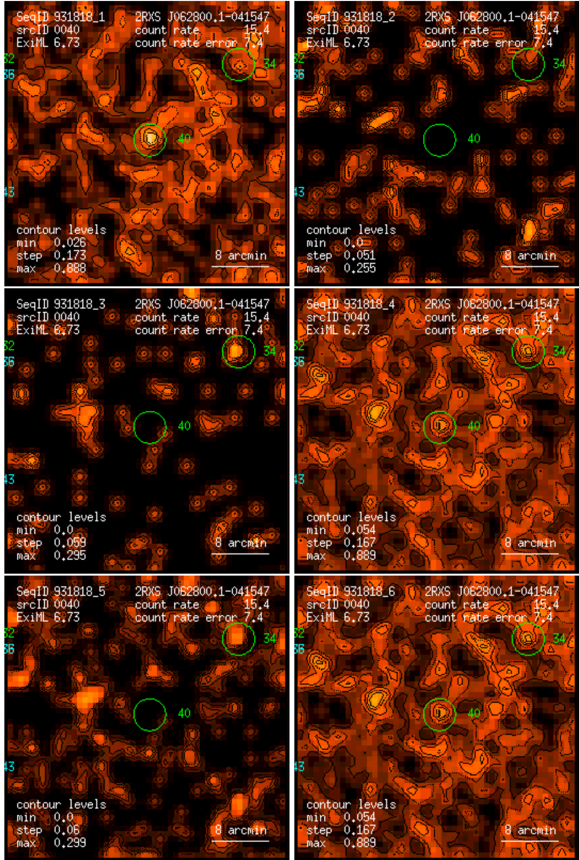
Figure 40: RASS 931818: detection 0040: band rate images, Gaussian filter: (1) PSPC channels 11 – 41, (2) 52 – 90, (3) 91 – 201, (4) 11 – 235, (5) 52 – 201, (6) 11 – 201. Broad band rates in counts/ks. Band rate contour levels in counts/ks/arcmin 2 .
