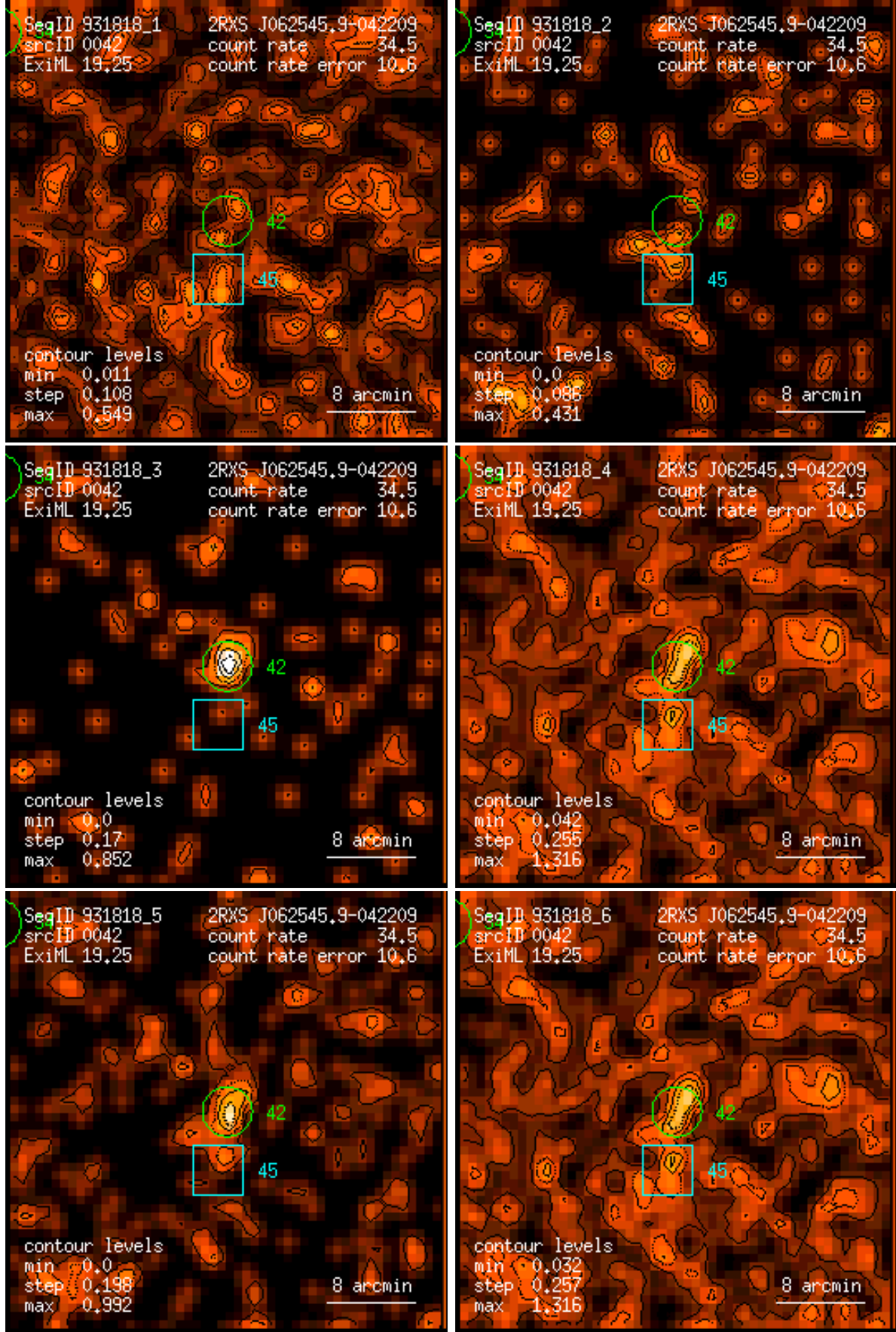
Figure 42: RASS 931818: detection 0042: band rate images, Gaussian filter: (1) PSPC channels 11 – 41, (2) 52 – 90, (3) 91 – 201, (4) 11 – 235, (5) 52 – 201, (6) 11 – 201. Broad band rates in counts/ks. Band rate contour levels in counts/ks/arcmin 2 .
