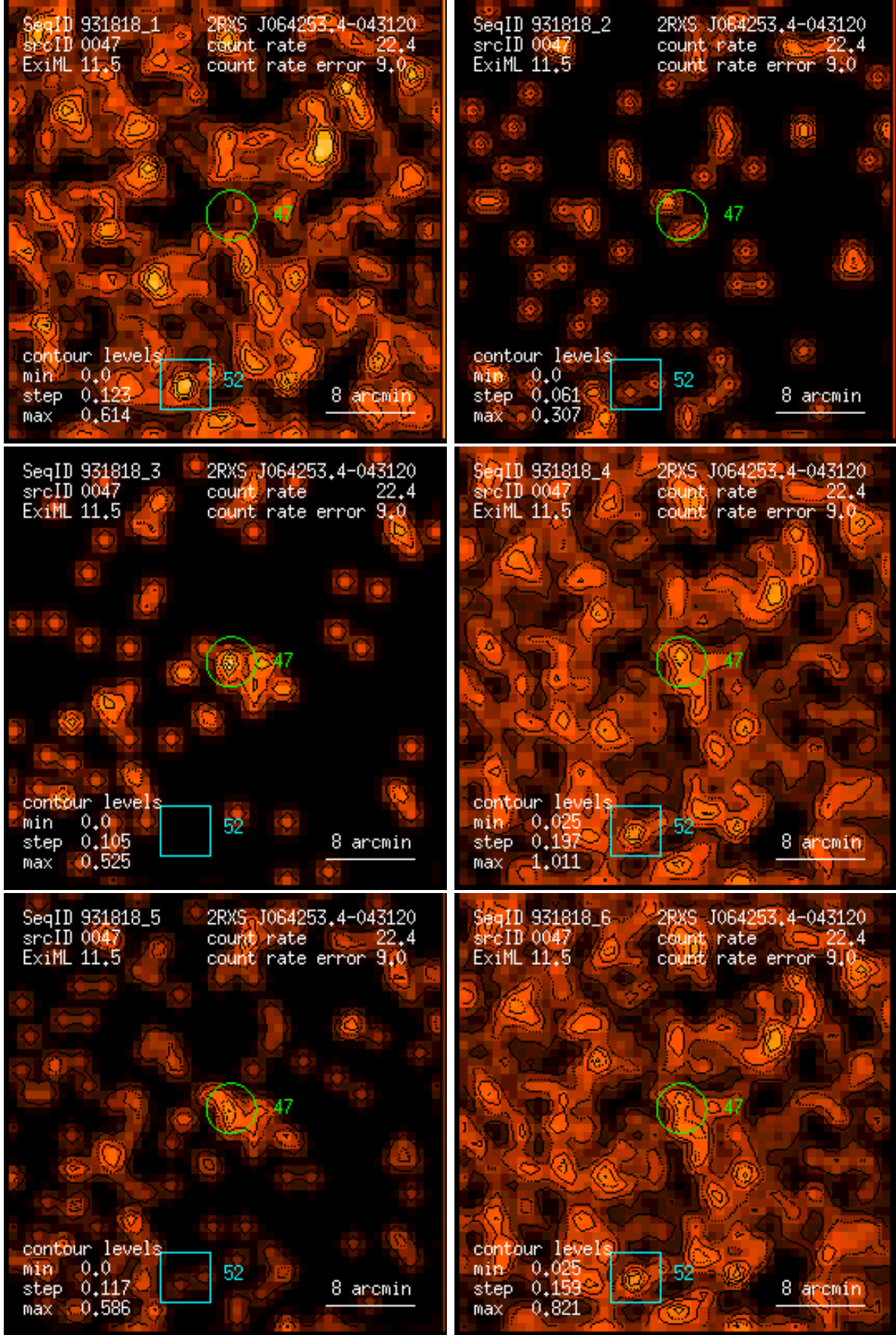
Figure 47: RASS 931818: detection 0047: band rate images, Gaussian filter: (1) PSPC channels 11 – 41, (2) 52 – 90, (3) 91 – 201, (4) 11 – 235, (5) 52 – 201, (6) 11 – 201. Broad band rates in counts/ks. Band rate contour levels in counts/ks/arcmin 2 .
