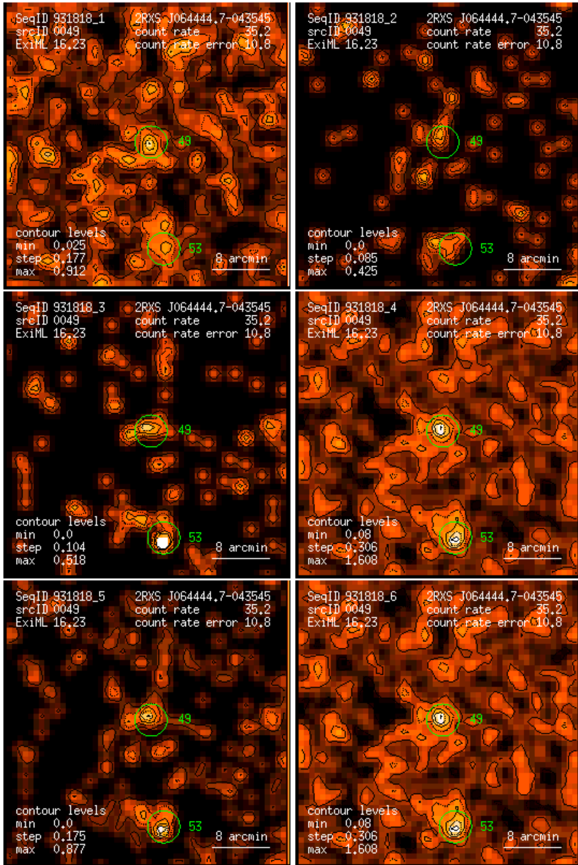
Figure 49: RASS 931818: detection 0049: band rate images, Gaussian filter: (1) PSPC channels 11 – 41, (2) 52 – 90, (3) 91 – 201, (4) 11 – 235, (5) 52 – 201, (6) 11 – 201. Broad band rates in counts/ks. Band rate contour levels in counts/ks/arcmin 2 .
