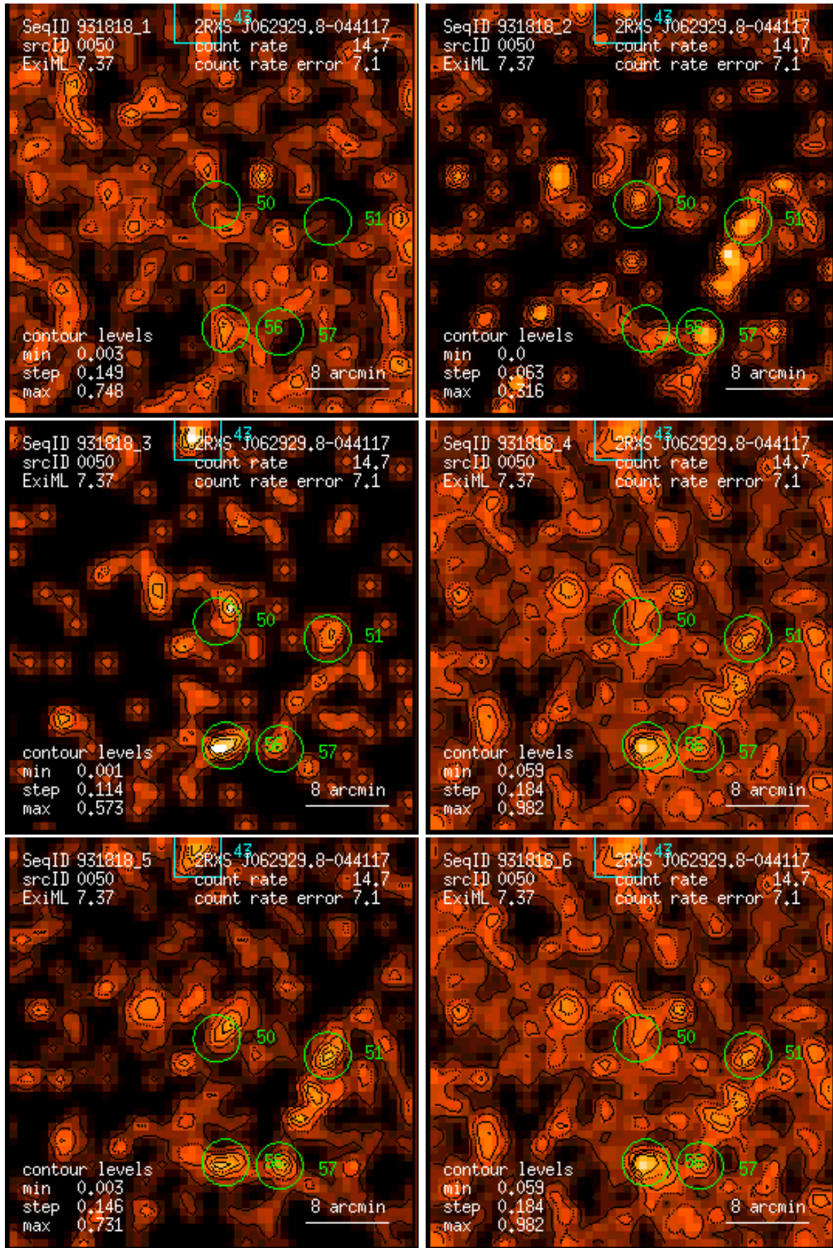
Figure 50: RASS 931818: detection 0050: band rate images, Gaussian filter: (1) PSPC channels 11 – 41, (2) 52 – 90, (3) 91 – 201, (4) 11 – 235, (5) 52 – 201, (6) 11 – 201. Broad band rates in counts/ks. Band rate contour levels in counts/ks/arcmin 2 .
