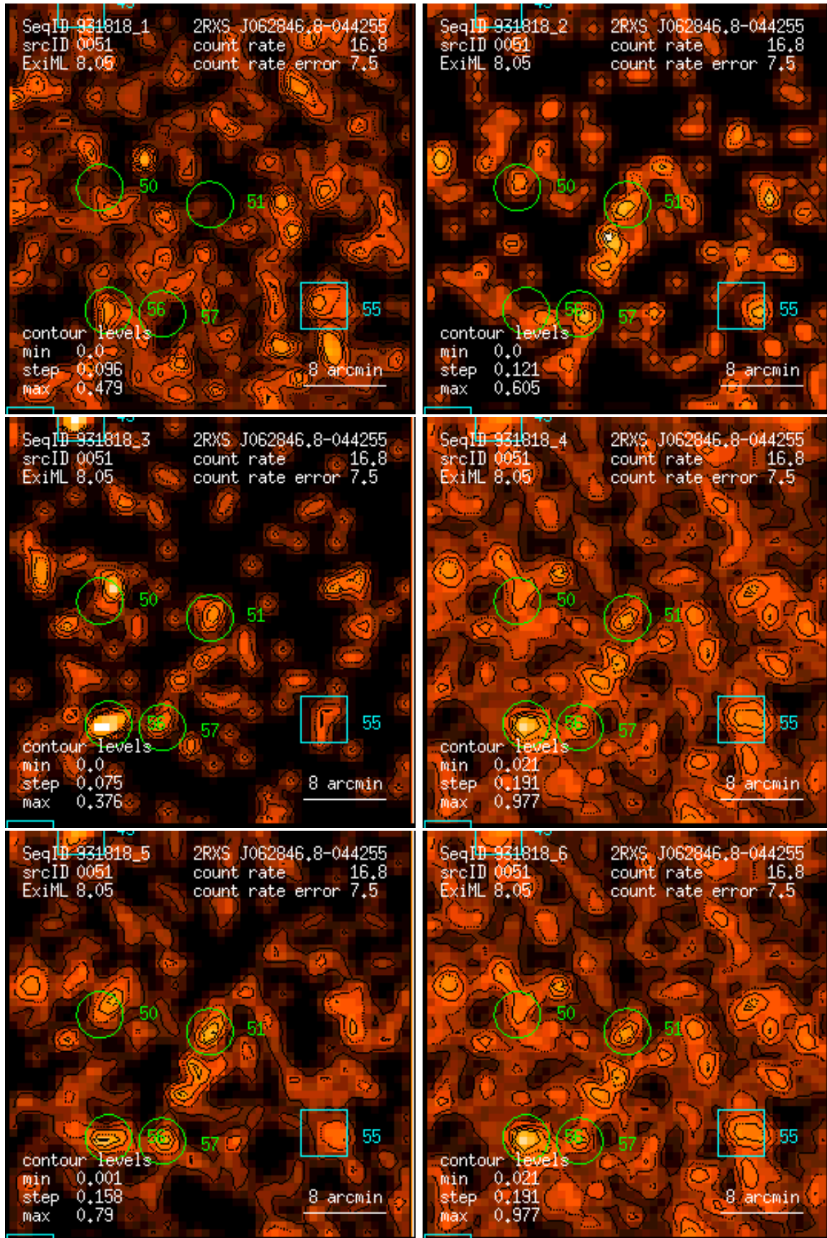
Figure 51: RASS 931818: detection 0051: band rate images, Gaussian filter: (1) PSPC channels 11 – 41, (2) 52 – 90, (3) 91 – 201, (4) 11 – 235, (5) 52 – 201, (6) 11 – 201. Broad band rates in counts/ks. Band rate contour levels in counts/ks/arcmin 2 .
